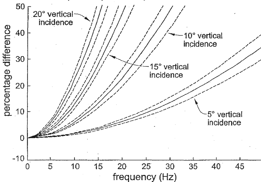
Fig. 8B Percentage difference between expected result and interpolated result (solid line) with standard difference (dashed lines) for monopole interpolation only.
