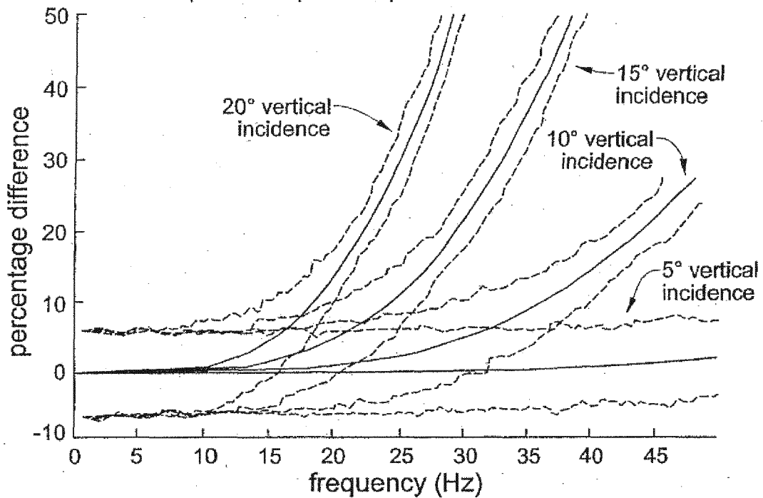
Fig. 8A Percentage difference between expected result and interpolated result (solid line) with standard deviation (dashed lines) for monopole and dipole interpolation.
