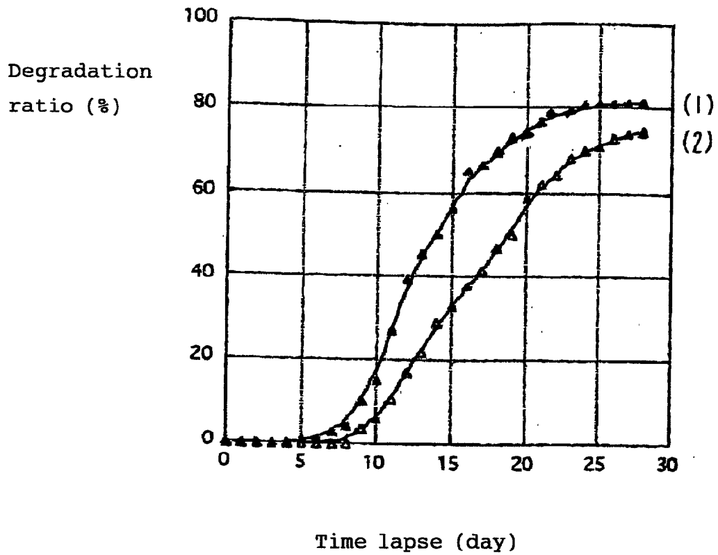
Evaluation of biodegradability by active sludge
