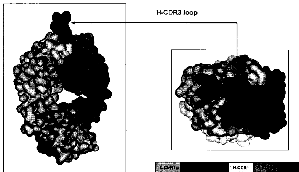
Figure 2. X-ray structure of AIN457 Fab, overall view
