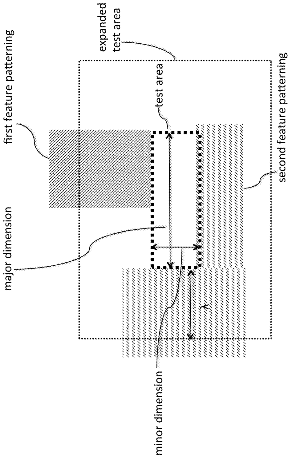
L-shape interlayer short (example 2)
