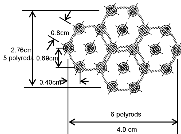
Proposed scalable Phased 4 Cell Array Unit
