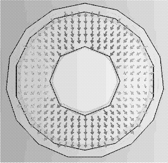
HE11, Horizontal Polarization
