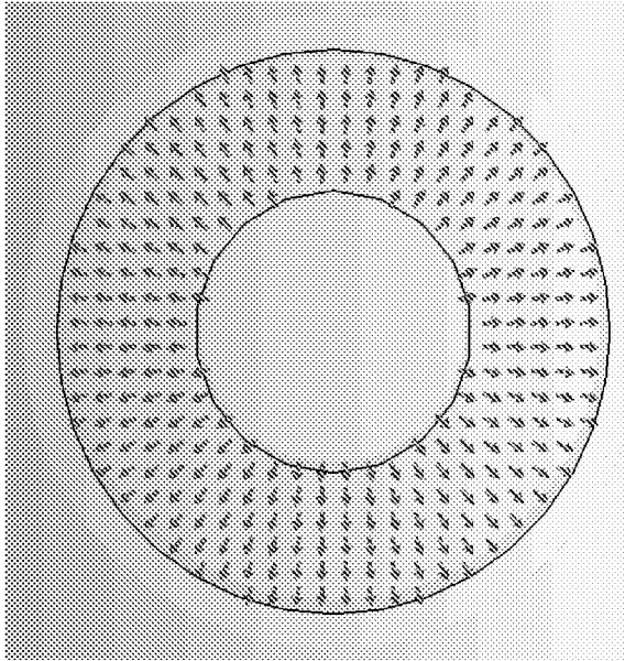
TM00 (Unpolarized)
