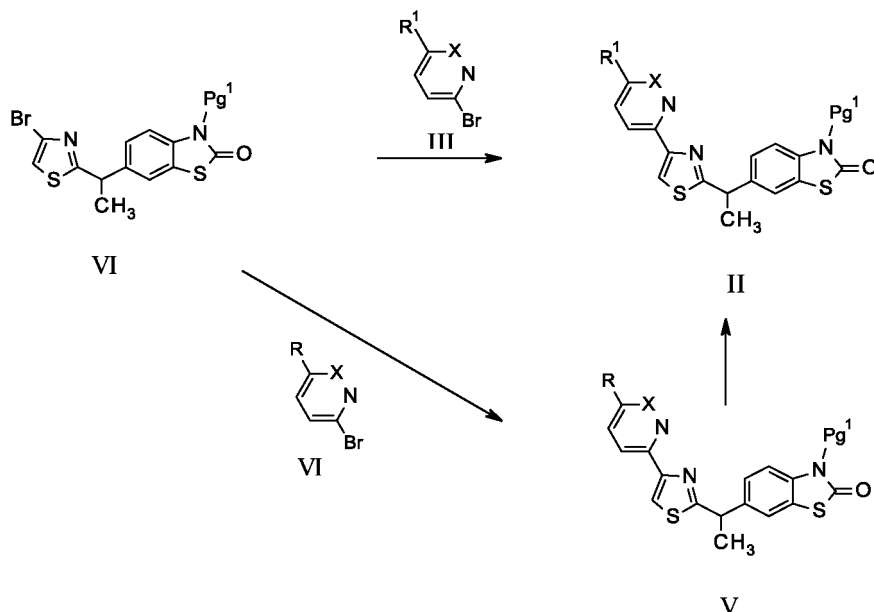
Scheme 3
