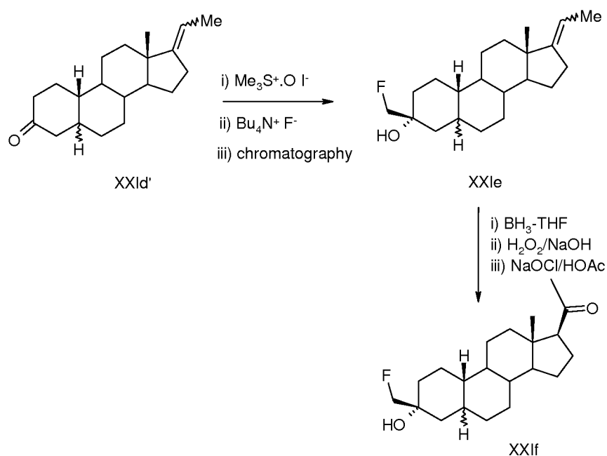
Scheme 2. Exemplary synthesis of 3 \beta -Fluoromethyl-3 \alpha -hydroxy-19-nor-pregnan-20-one
