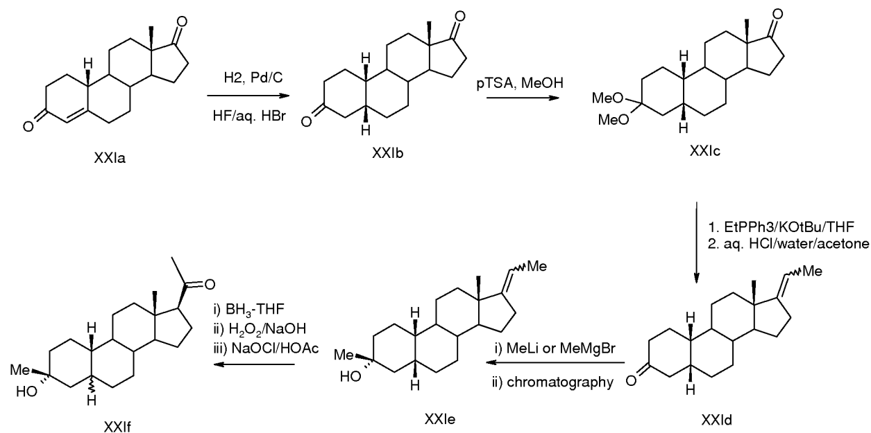
Scheme 1. Exemplary synthesis of 3 \beta -Methyl-3 \alpha -hydroxy-19-nor-pregnan-20-one
