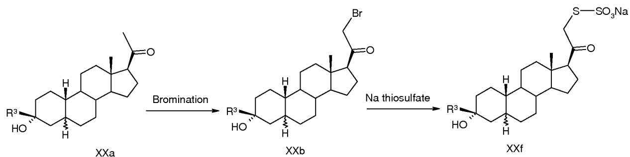
Scheme 11. Exemplary synthesis of 19-norpregnane 21-thiosulfates
