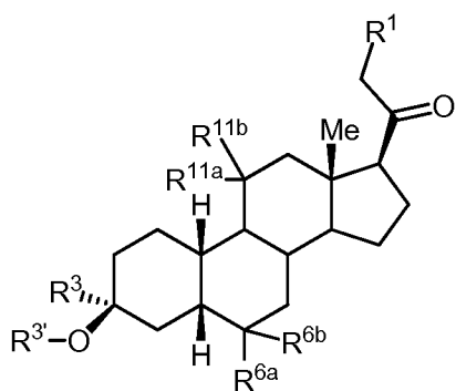
(III-b1)
