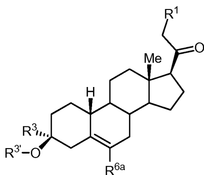
(III-c3)
