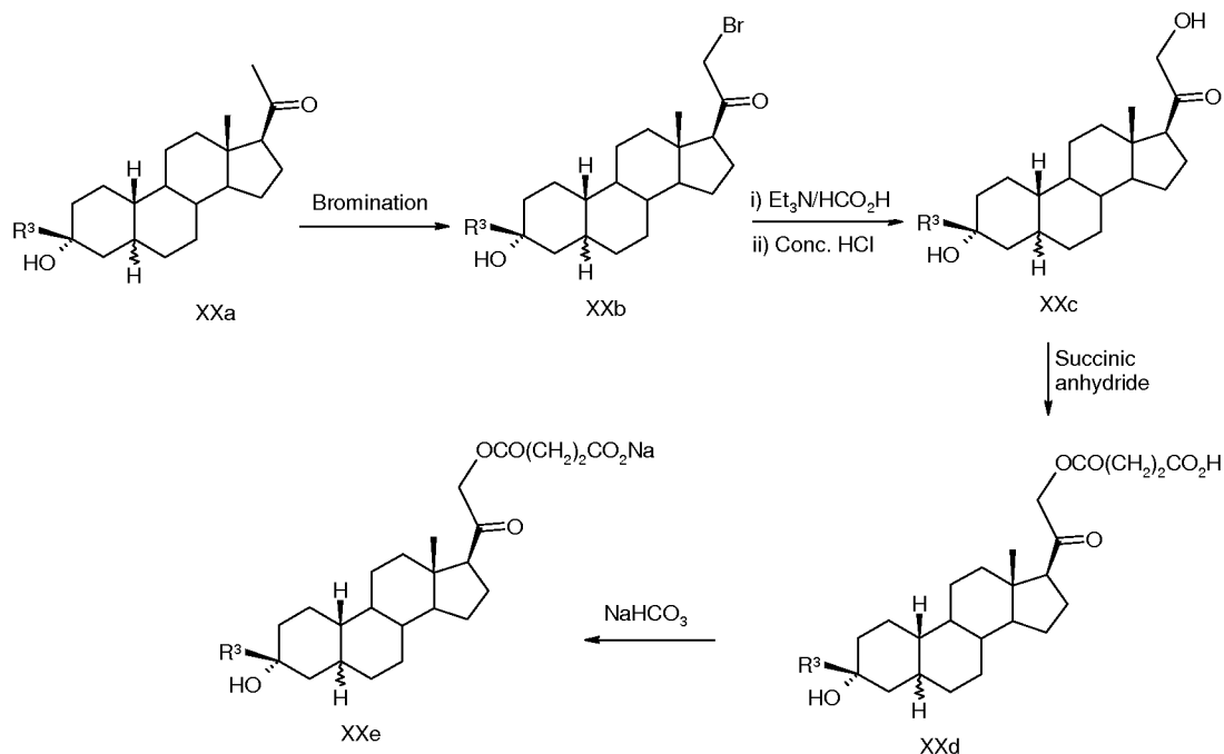
Scheme 10. Exemplary synthesis of 21-hydroxy and 21-hemisuccinate 19-norpregnanes
