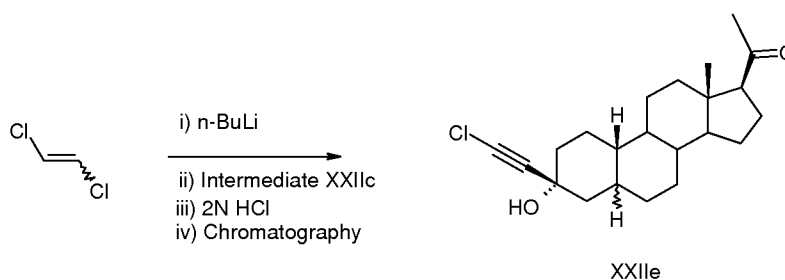
Scheme 6. Exemplary synthesis of 3 \beta -Cyclopropylethynyl-3 \alpha -hydroxy-19-nor-pregnan-20-one
