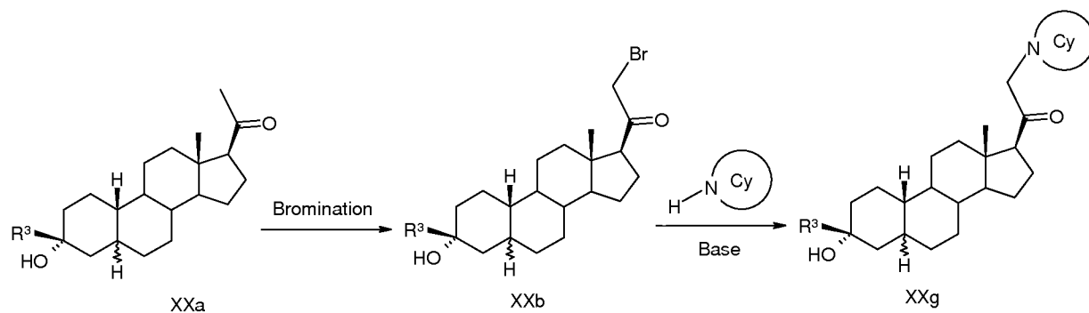
Scheme 12. Exemplary synthesis of 21-heteroaryl 19-nor pregnanes
