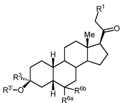
(III-c1)
