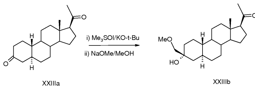
Scheme 9. Exemplary synthesis of 3 \beta -Trifluoroethynyl-3 \alpha -hydroxy-19-nor-pregnan-20-one
