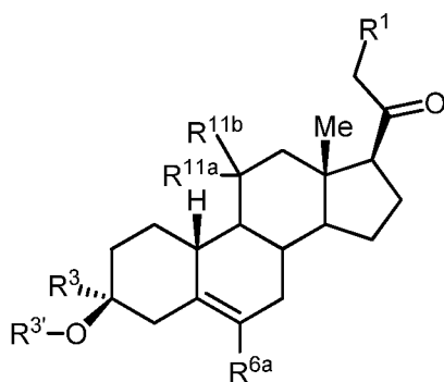
(III-b3)
