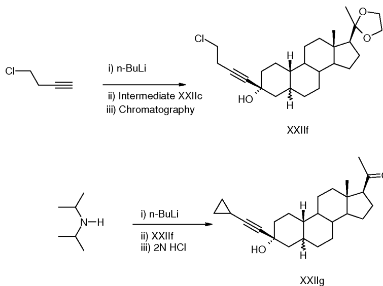
Scheme 6. Exemplary synthesis of 3 \beta -Cyclopropylethynyl-3 \alpha -hydroxy-19-nor-pregnan-20-one
