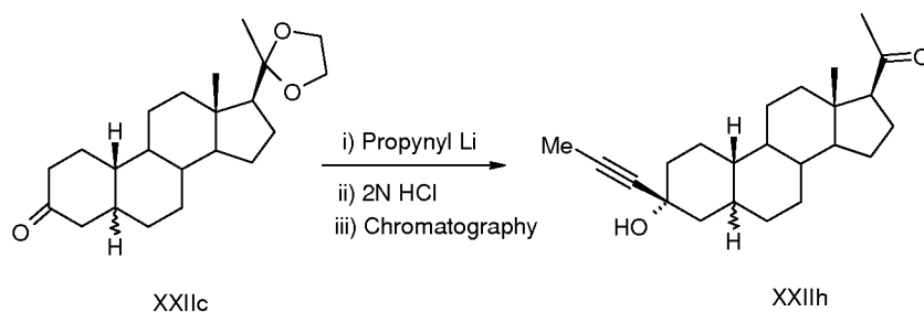
Scheme 8. Exemplary synthesis of 3 \beta -Methoxymethyl-3 \alpha -hydroxy-19-nor-pregnan-20-one
