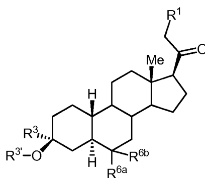
(III-c1)
