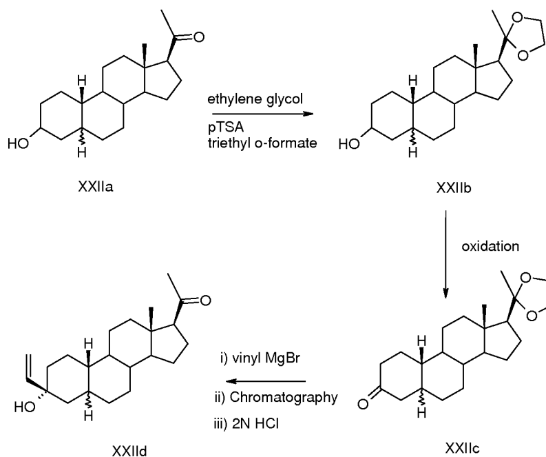
Scheme 4. Exemplary synthesis of 3 \beta -Ethenyl-3 \alpha -hydroxy-19-nor-pregnan-20-one
