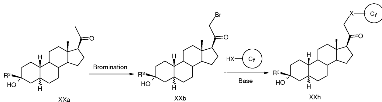
Scheme 13. Exemplary synthesis of 21-heteroaryloxy/thiooxy 19-nor pregnanes
