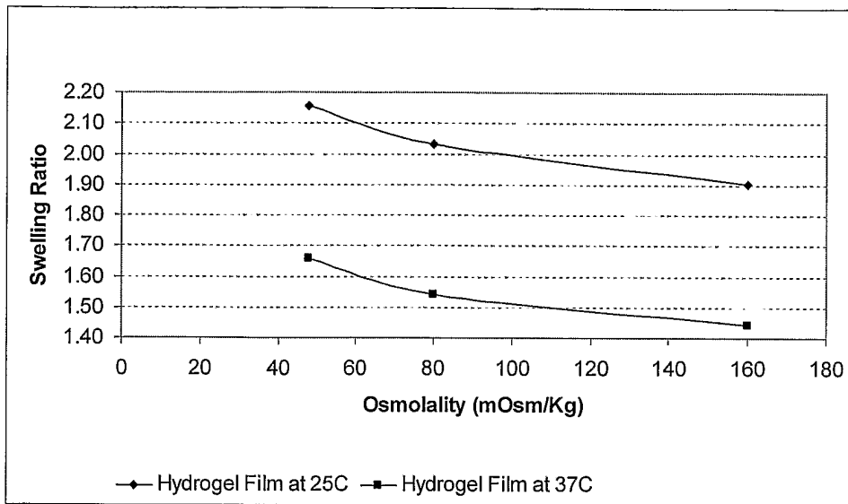
Figure 15. Plot of swelling ratio of hydroxypropyl acrylate/acrylamide hydrogel versus osmolality.
