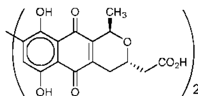
actinorhodine (VI),
