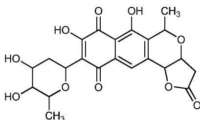
Derivative 1 (VII)
