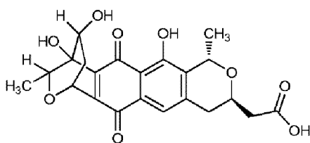
Derivat 2 (VIII),
