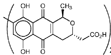
Actinorhodin (VI),
