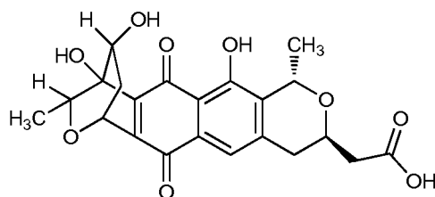
Derivative 2 (VIII),
