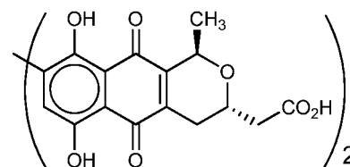
actinorhodin (VI),
