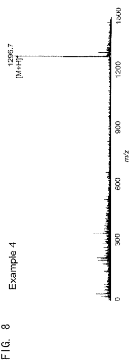
Mass spectrum of angiotensin-I measured in Example 4
