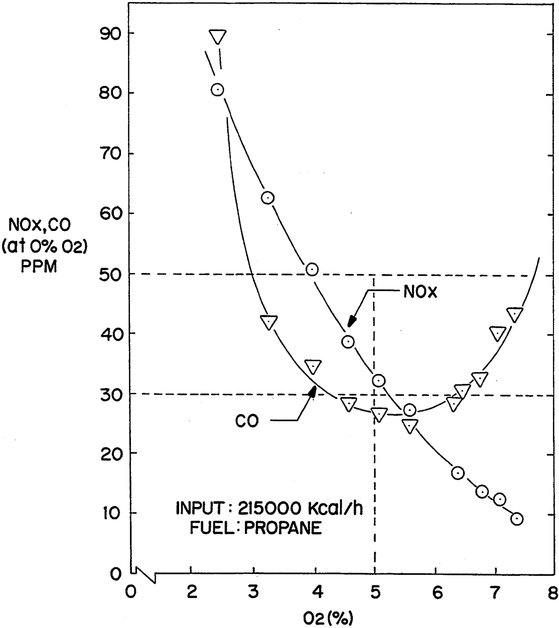
FIG. 9 PRIOR ART
