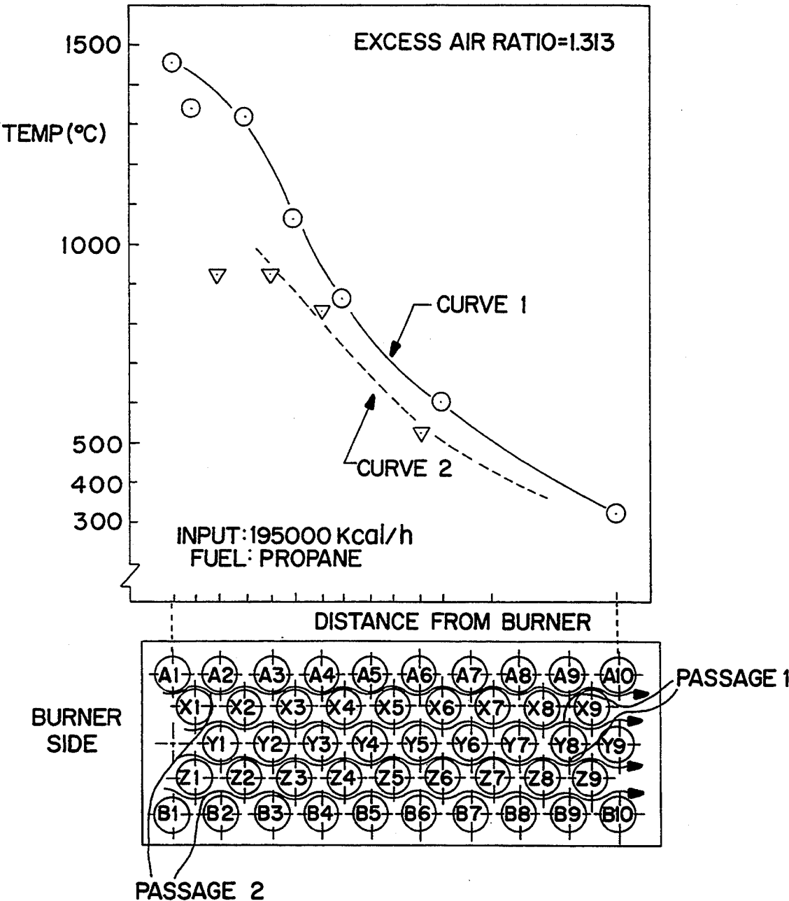
FIG. 12 PRIOR ART
