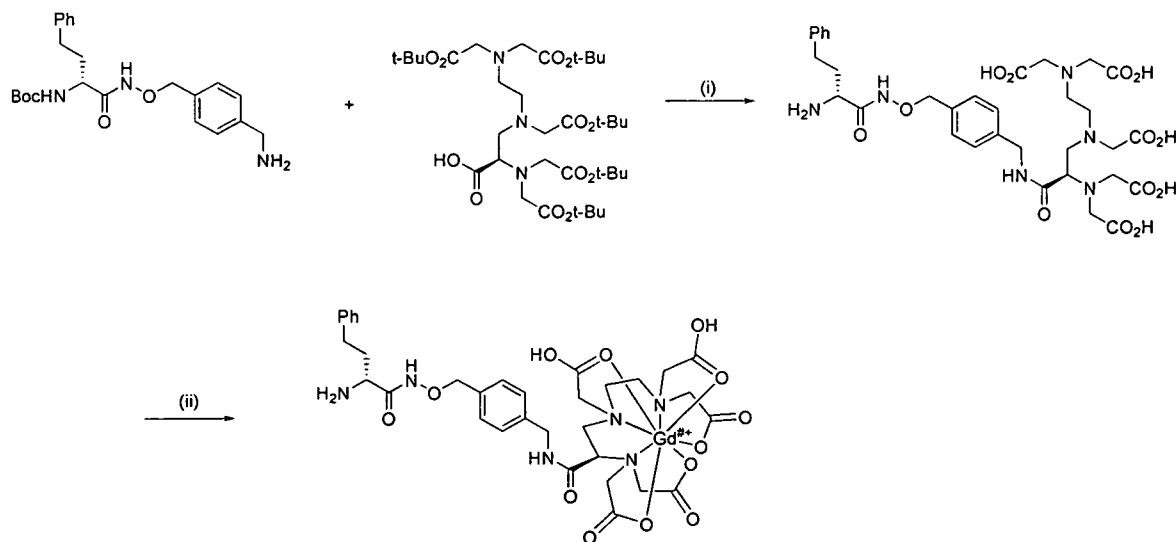
Scheme 4
