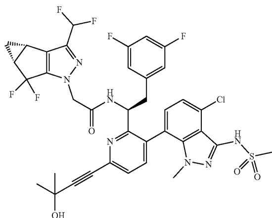
Compound A
