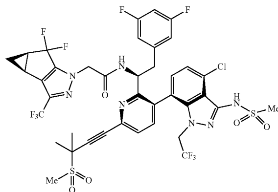
Isomer A
