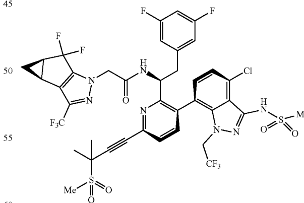
Isomer B
