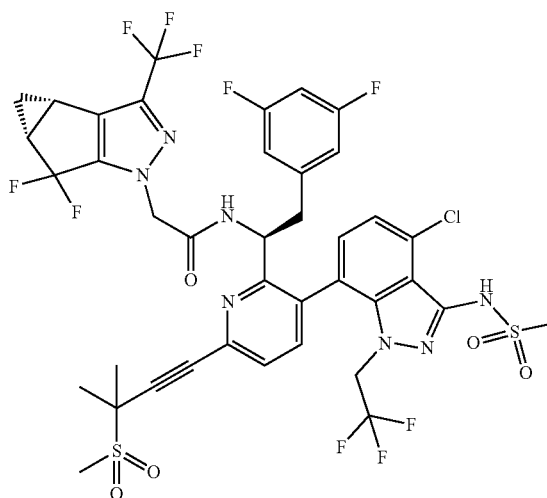
Compound 1
