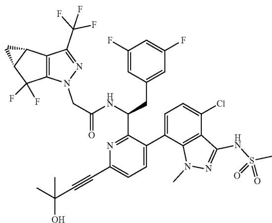
Compound B
