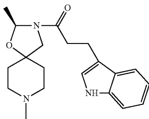
((S)-1-(2,8-dimethyl-1-oxa-3,8-diazaspiro[4.5]dec-3-yl)-3-(1H-indol-3-yl)-propan-1-one)
