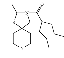
(1-(2,8-dimethyl-1-thia-3,8-diazaspiro[4.5]dec-3-yl)-2-propylpentan-1-one),
