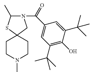
((3,5-di-tert-butyl-4-hydroxy-phenyl)-(2,8-dimethyl-1-thia-3,8-diazaspiro[4.5]dec-3-yl)-methanone),
