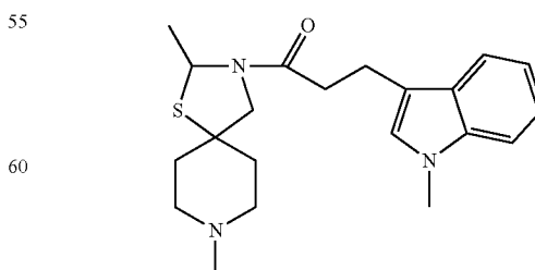
1-(2,8-Dimethyl-1-thia-3,8-diazaspiro[4.5]dec-3-yl)-3-(1-methylindol-3-yl)propan-1-one,
