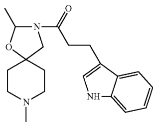
1-(2,8-dimethyl-1-oxa-3,8-diazaspiro[4.5]dec-3-yl)-3-(1H-indol-3-yl)-propan-1-one,
