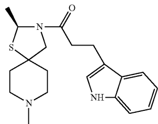
((S)-1-(2,8-dimethyl-1-thia-3,8-diazaspiro[4.5]dec-3-yl)-3-(1H-indol-3-yl)propan-1-one) (AF710B),
