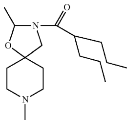
(1-(2,8-dimethyl-1-oxa-3,8-diazaspiro[4.5]dec-3-yl)-2-propyl-pentan-1-one),
