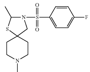
(3-(4-fluorobenzenesulfonyl)-2,8-dimethyl-1-thia-3,8-diazaspiro[4.5]decane),
