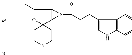
(1',4-dimethyl-6-(3-indolpropionyl)-spiro-(3-oxa-6-aza-bicyclo[3.1.0]hexane-2,4'-piperidine)), and
