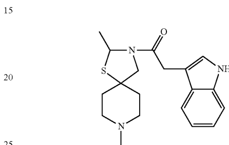
(1-(2,8-dimethyl-1-thia-3,8-diazaspiro[4.5]dec-3-yl)-2-(1H-indol-3-yl)ethan-1-one),
