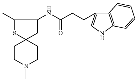
N-(2,8-Dimethyl-1-thia-8-aza-spiro[4.5]dec-3-yl)-3-(1H-indol-3-yl)-propanamide,
