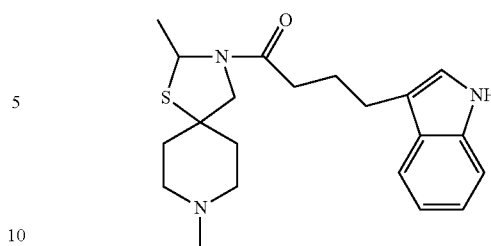
(1-(2,8-dimethyl-1-thia-3,8-diazaspiro[4.5]dec-3-yl)-4-(1H-indol-3-yl)butan-1-one),
