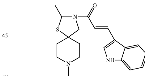
(1-(2,8-dimethyl-1-thia-3,8-diazaspiro[4.5]dec-3-yl)-3-(1H-indol-3-yl)prop-2-ene-1-one),
