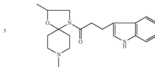
(1-(2,8-dimethyl-1-oxa-4,8-diazaspiro[4.5]dec-4-yl)-3-(1H-indol-3-yl)-propan-1-one),
