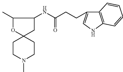
N-(2,8-dimethyl-1-oxa-8-aza-spiro[4.5]dec-3-yl)-3-(1H-indol-3-yl)-propanamide,
