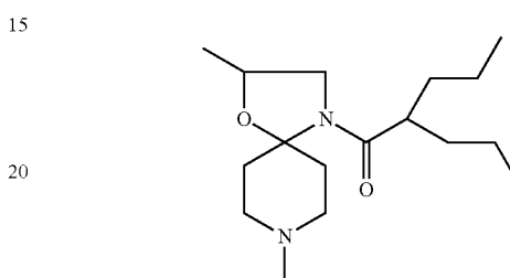
(1-(2,8-dimethyl-1-oxa-4,8-diazaspiro[4.5]dec-4-yl)-2-propyl-pentan-1-one),
