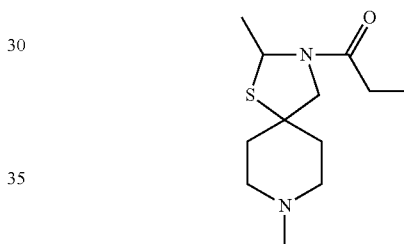
(1-(2,8-dimethyl-1-thia-3,8-diazaspiro[4.5]dec-3-yl)-propan-1-one),
