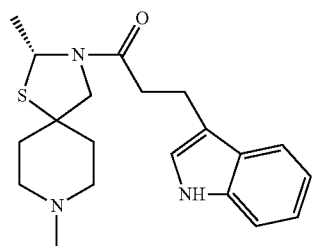
((R)-1-(2,8-dimethyl-1-thia-3,8-diazaspiro[4.5]dec-3-yl)-3-(1H-indol-3-yl)propan-1-one),
