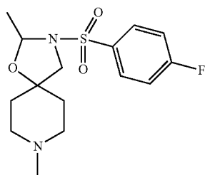
(3-(4-fluorobenzenesulfonyl)-2,8-dimethyl-1-oxa-3,8-diazaspiro[4.5]-decane),
