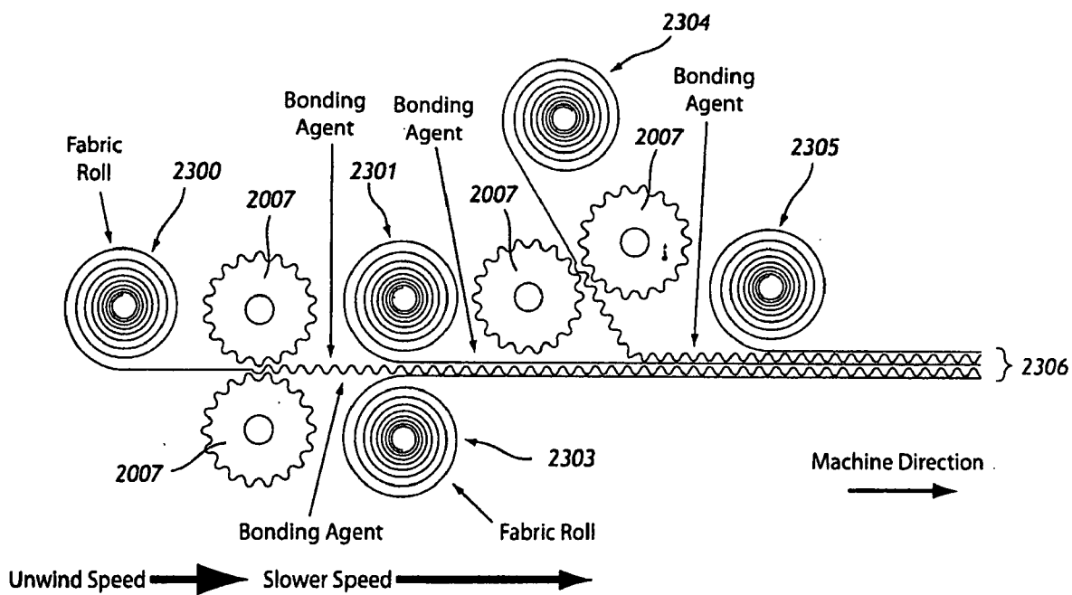
Figure 4 (Prior Art)
