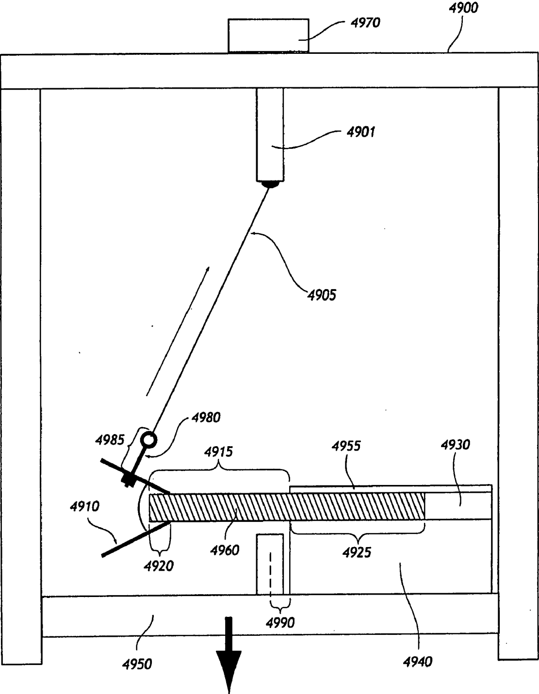
Figure 49 - Bending Force Tester
