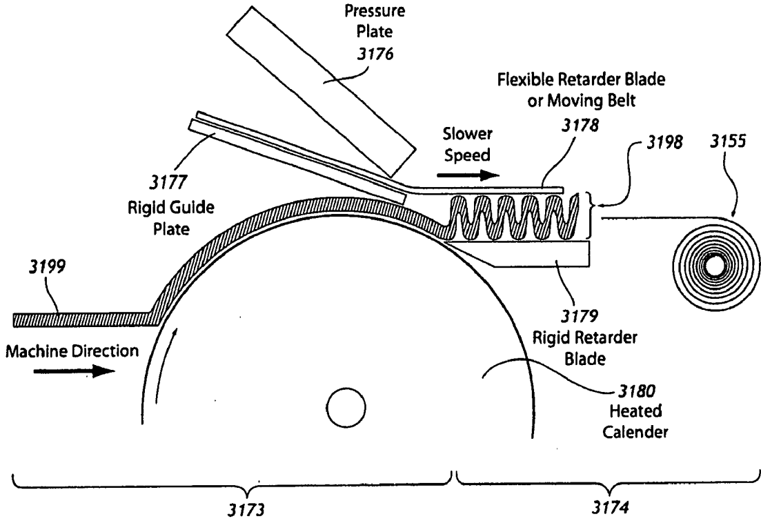
Figure 31B (Micrex® Microcreping)
