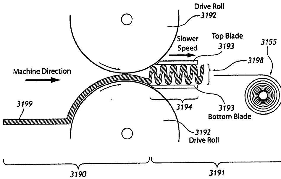
Figure 31C (Micrex® Microcreping)
