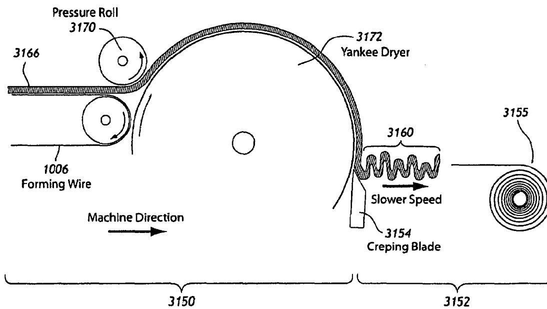
Figure 31A (Creping)
