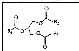
Formula 1. Structure of triglyceride
