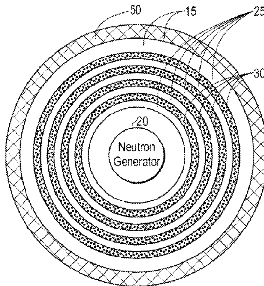
Cross-Section of Circle or Cylinder
