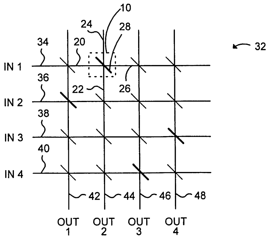
FIG. 2 (PRIOR ART)
