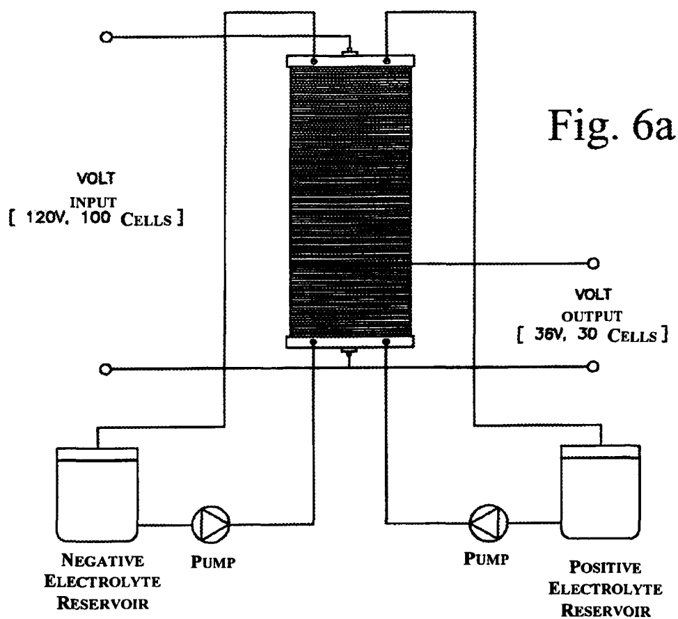
SELF-TRANSFORMER FOR DC CURRENTS
