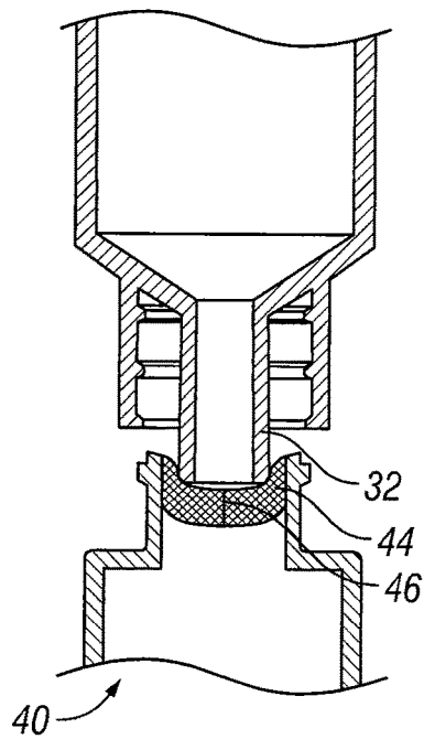
FIG. 3C (Prior Art)
