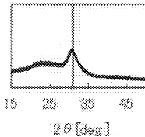
FIG. 23A Sample X1: 170°C, O 2 ≈30%
