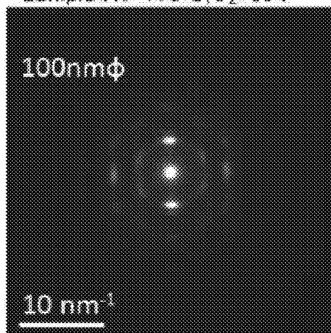
FIG. 23C Sample X1: 170°C, O 2 ≈30%
