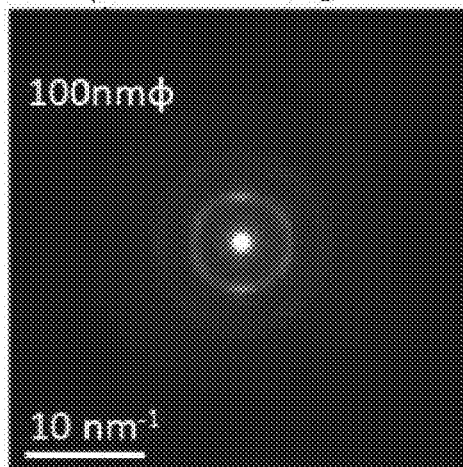
FIG. 24C Sample X2: 130°C, O 2 ≈10%
