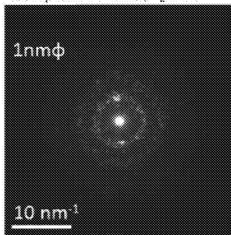
FIG. 24B Sample X2: 130°C, O 2 ≈10%
