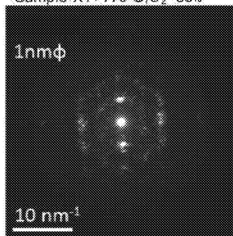
FIG. 23B Sample X1: 170°C, O 2 ≈30%
