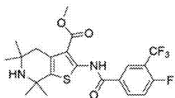
GP1-19; MW = 458
