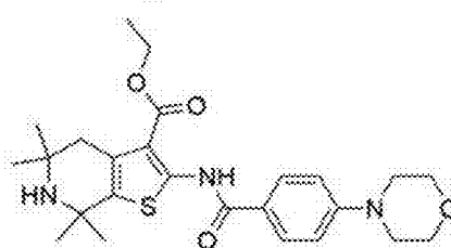
RS1-199; MW = 471
