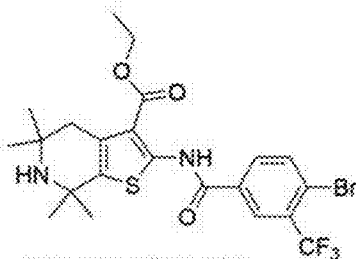
RS1-198; MW = 533
