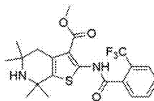
GP1-22; MW = 440
