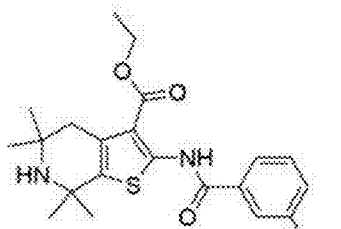
RS1-200; MW = 512
