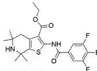
RS1-202; MW = 440
