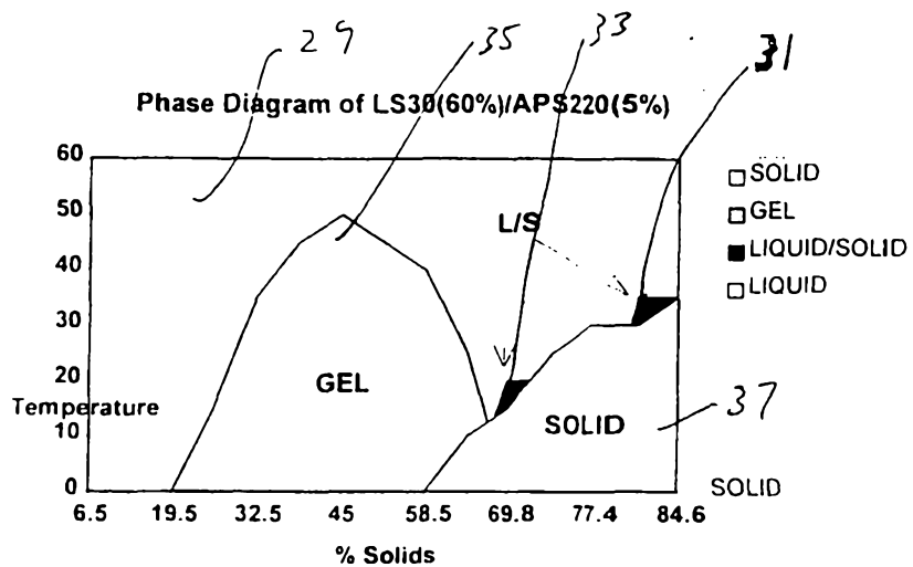
Figure 3 The Phase Diagram of the LS30 ( 60% ) / APS 220 ( 5% ) / water ( 35% ) blend
