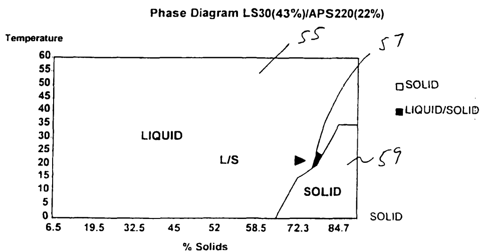
Figure 6 The Phase Diagram of the LS30 ( 43% ) / APS 220 ( 22% ) Blend
