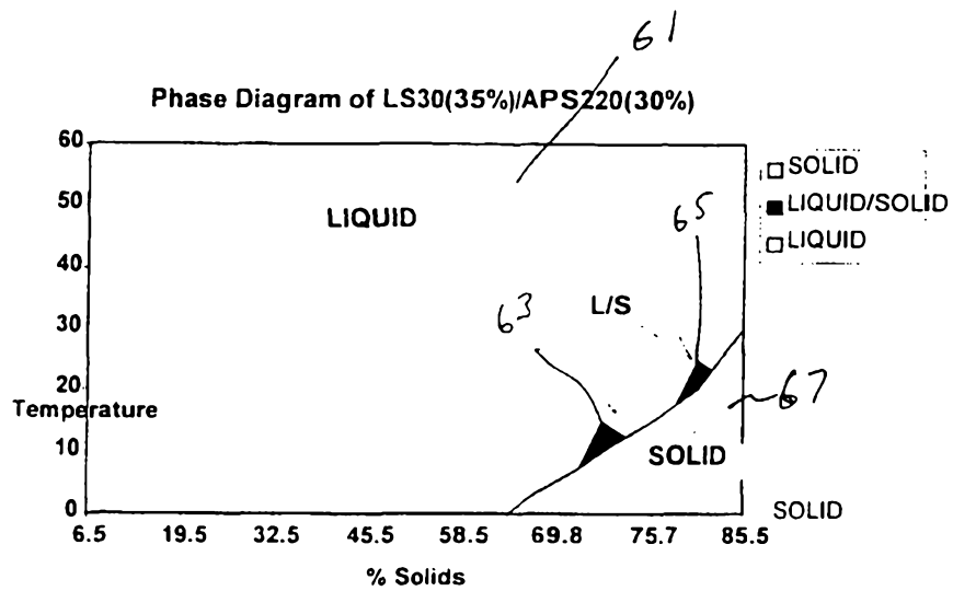
Figure 7 The Phase diagram of LS30 ( 35% ) / APS 220 (30%) / water ( 25%)
