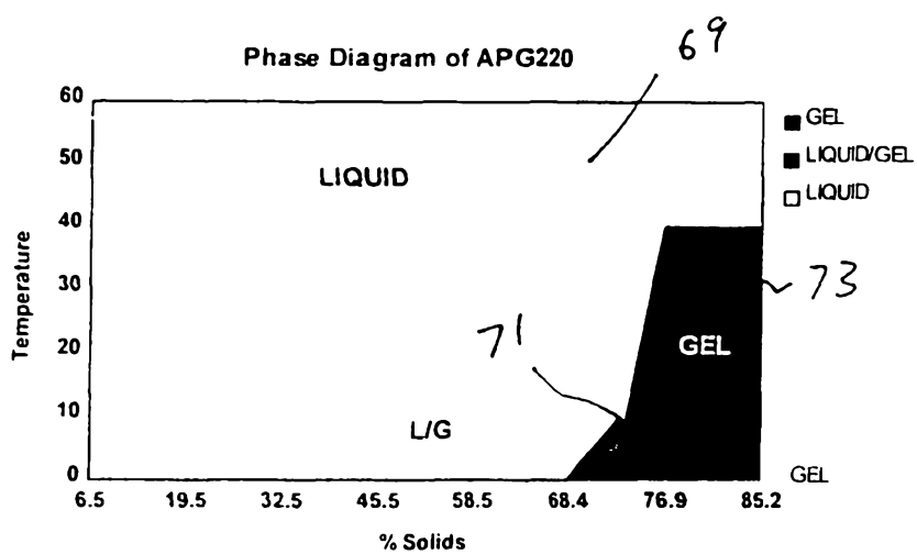
Figure 8 The Phase Diagram of APS 220 and Water
