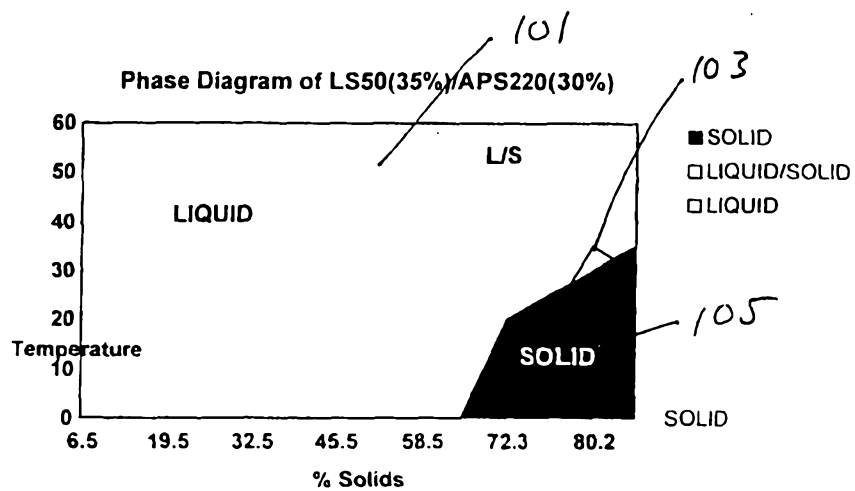
Figure 12 Phase Diagram of 35% LS50/ 30% APS 220/ 35% water
