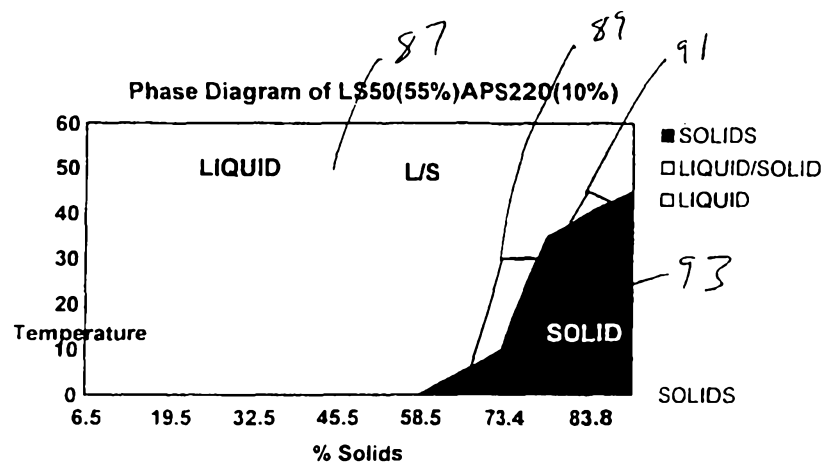
Figure 10 Phase Diagram of 55% LS50/ 10% APS 220/ 35% water
