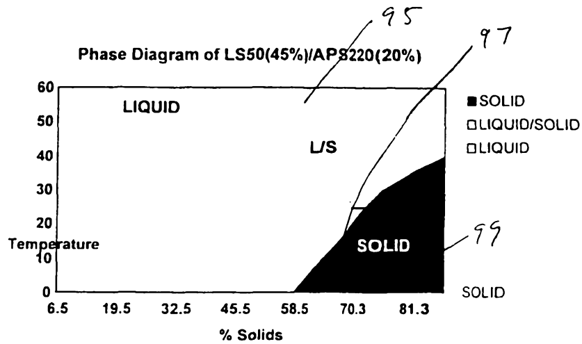
Figure 11 Phase Diagram of 45% LS50/ 20% APS 220/ 35% water
