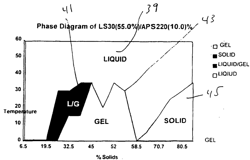
Figure 4 The phase diagram of the LS30 ( 55% ) / APS 220 ( 10% ) Blend
