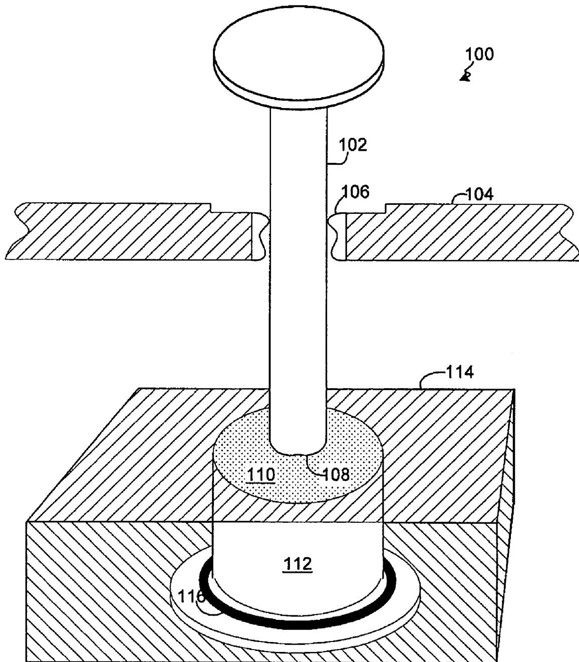
FIG. 1 (PRIOR ART)
