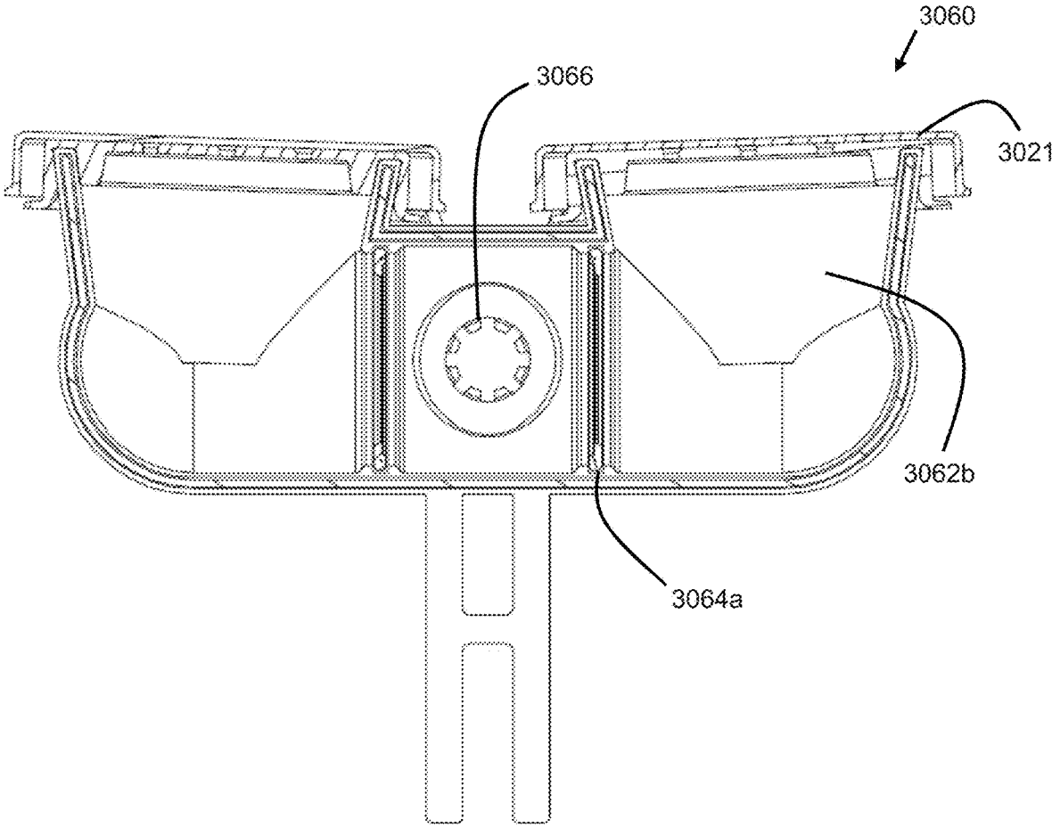
SECTION B-B
