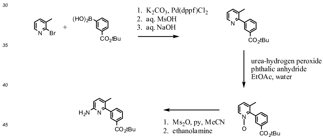
Scheme 2. Synthesis of the amine moiety.
