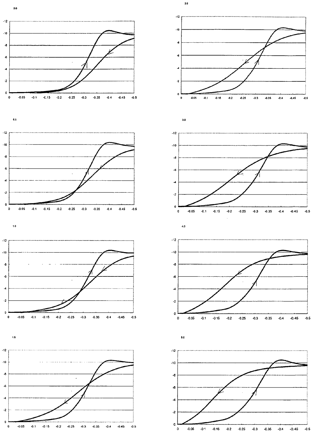
Figure 8. Voltammograms for PC 75 copper bath showing a hysteresis in copper reduction for various concentration of brightener.
