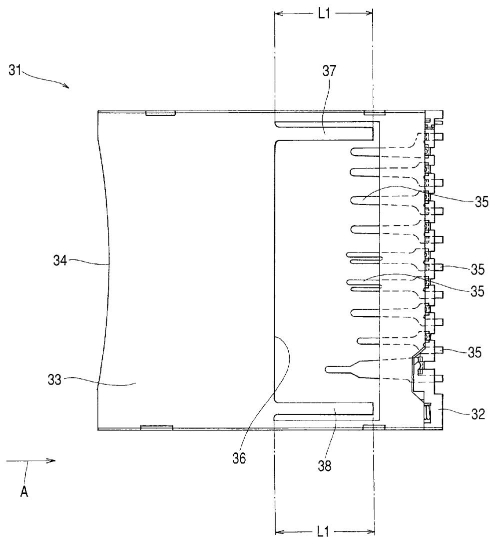
FIG. 14 PRIOR ART
