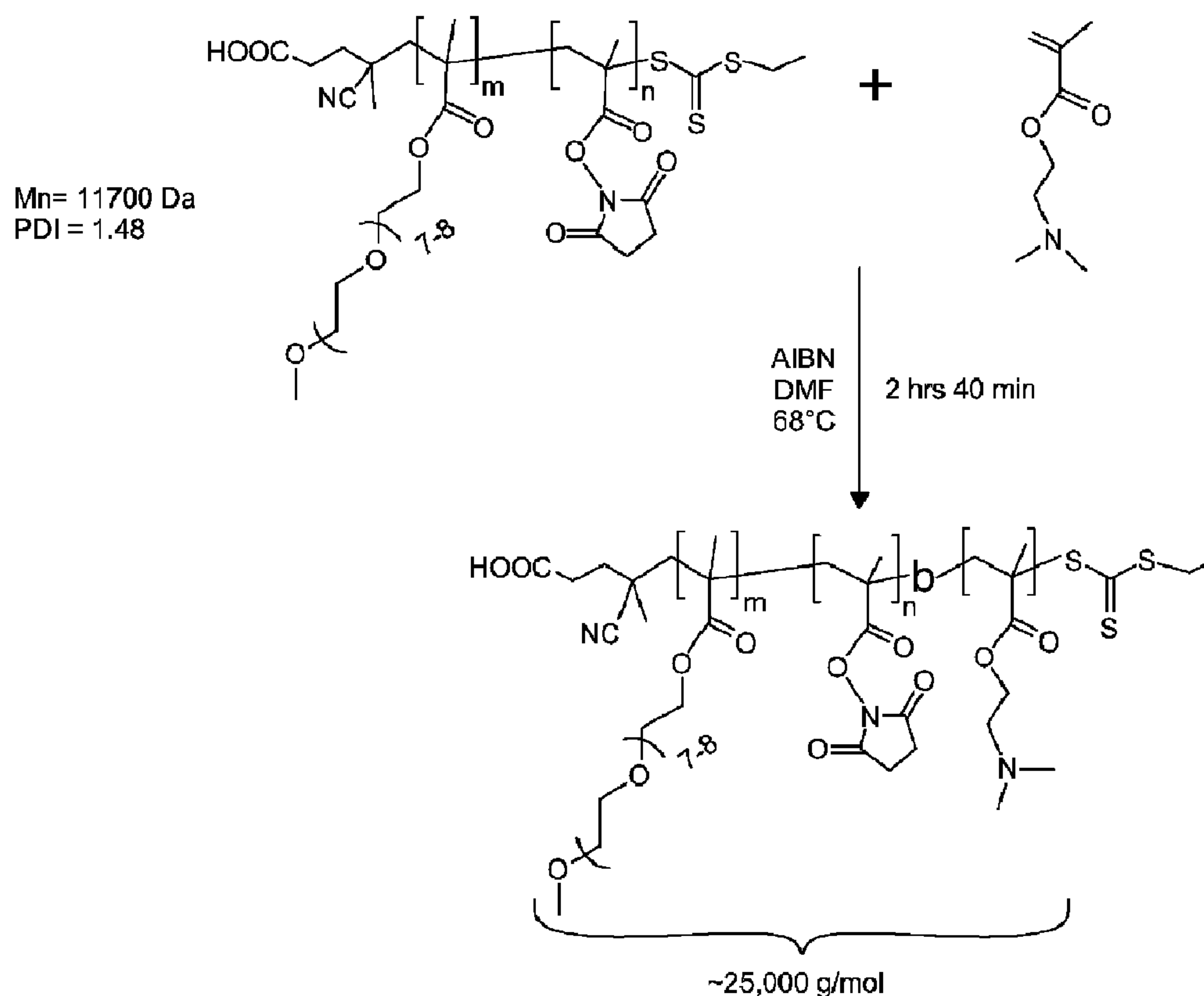
Fig. 1 Synthesis of poly(PEGMA-MANHS)-b-(DMAEMA)
