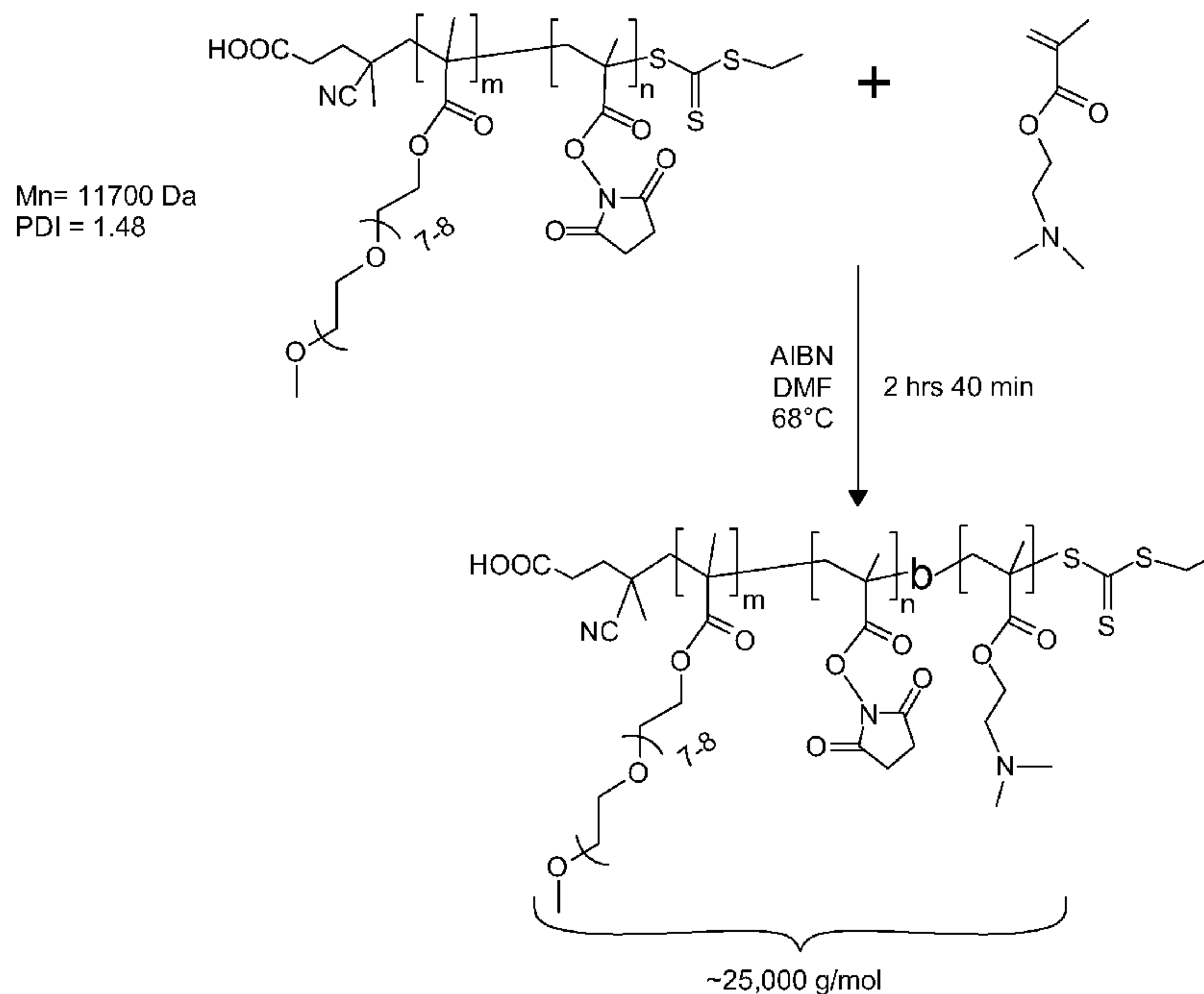
Fig. 1 Synthesis of poly(PEGMA-MANHS)-b-(DMAEMA)
