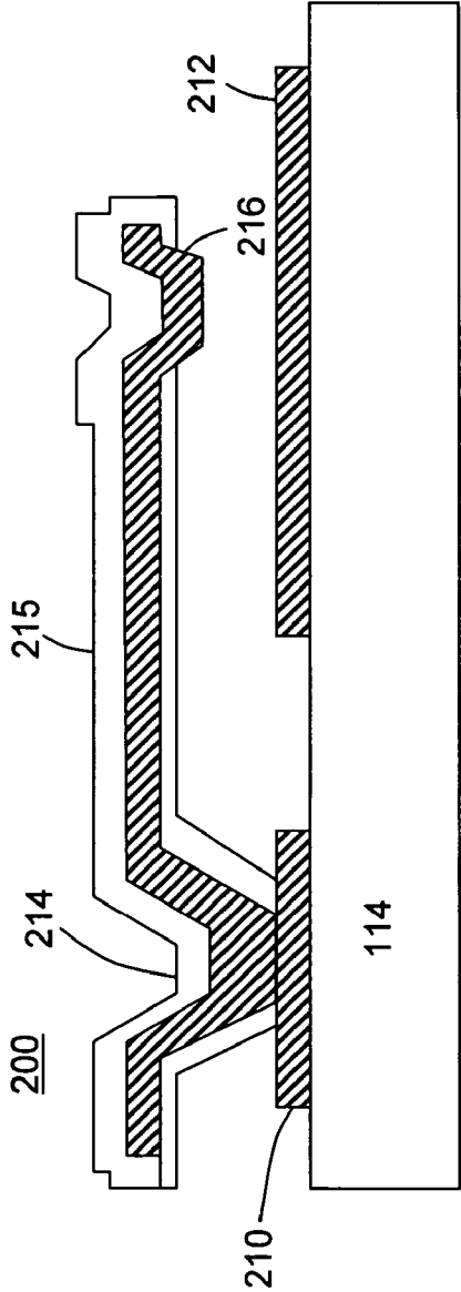
FIG. 2C PRIOR ART
