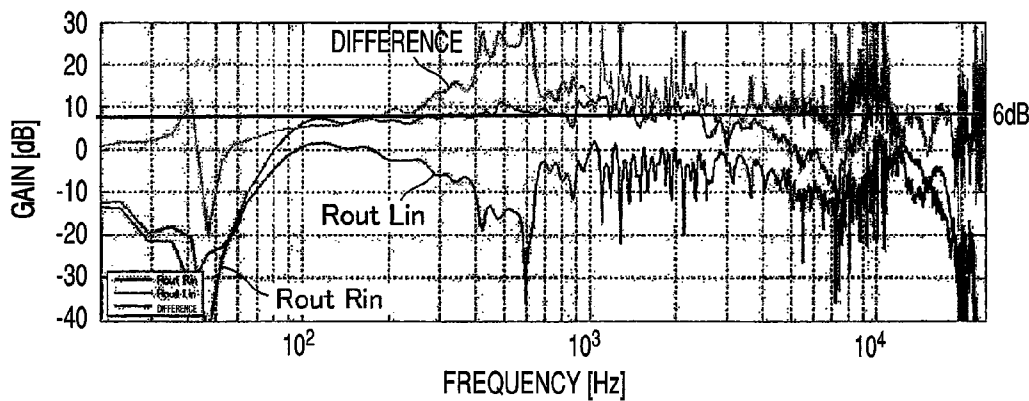
Rch LOUDSPEAKER OUT - AMPLITUDE CHARACTERISTIC
