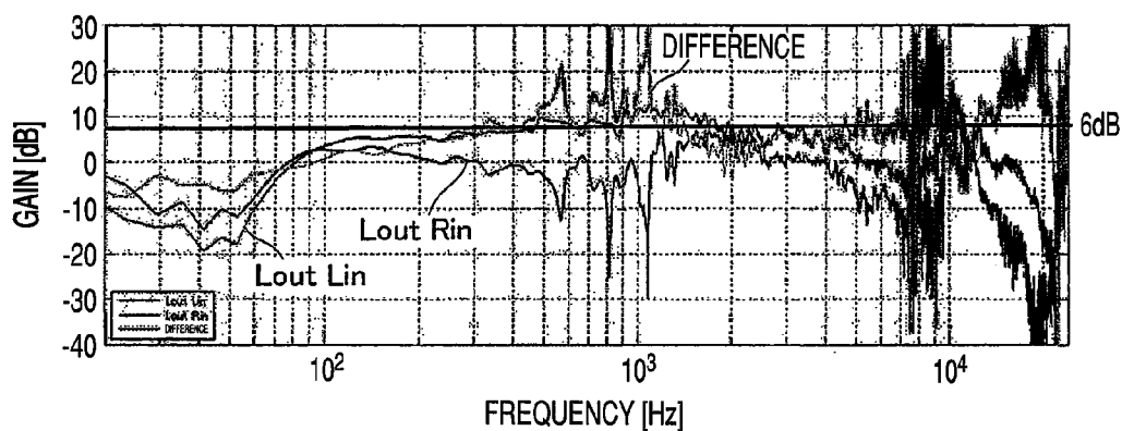
Lch LOUDSPEAKER OUT - AMPLITUDE CHARACTERISTIC
