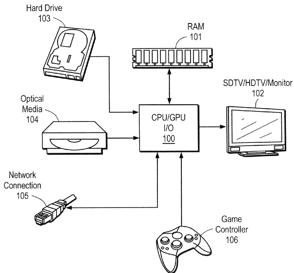
FIG. 1 (Prior Art)
