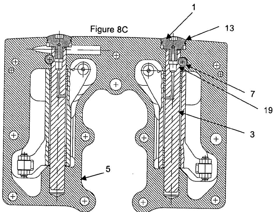
SECTION B-B
