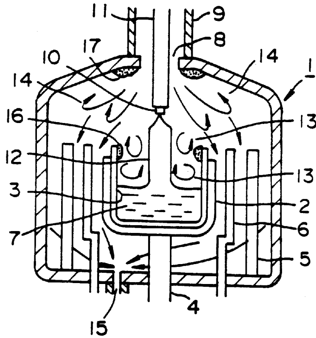
FIG. 4 (PRIOR ART)
