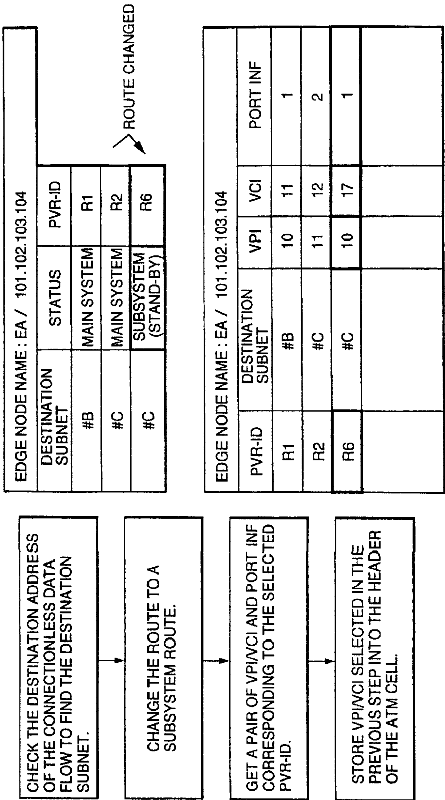
ROUTING TABLE SEARCH AND SETUP PROCEDURE USED IN EDGE NODE EA
