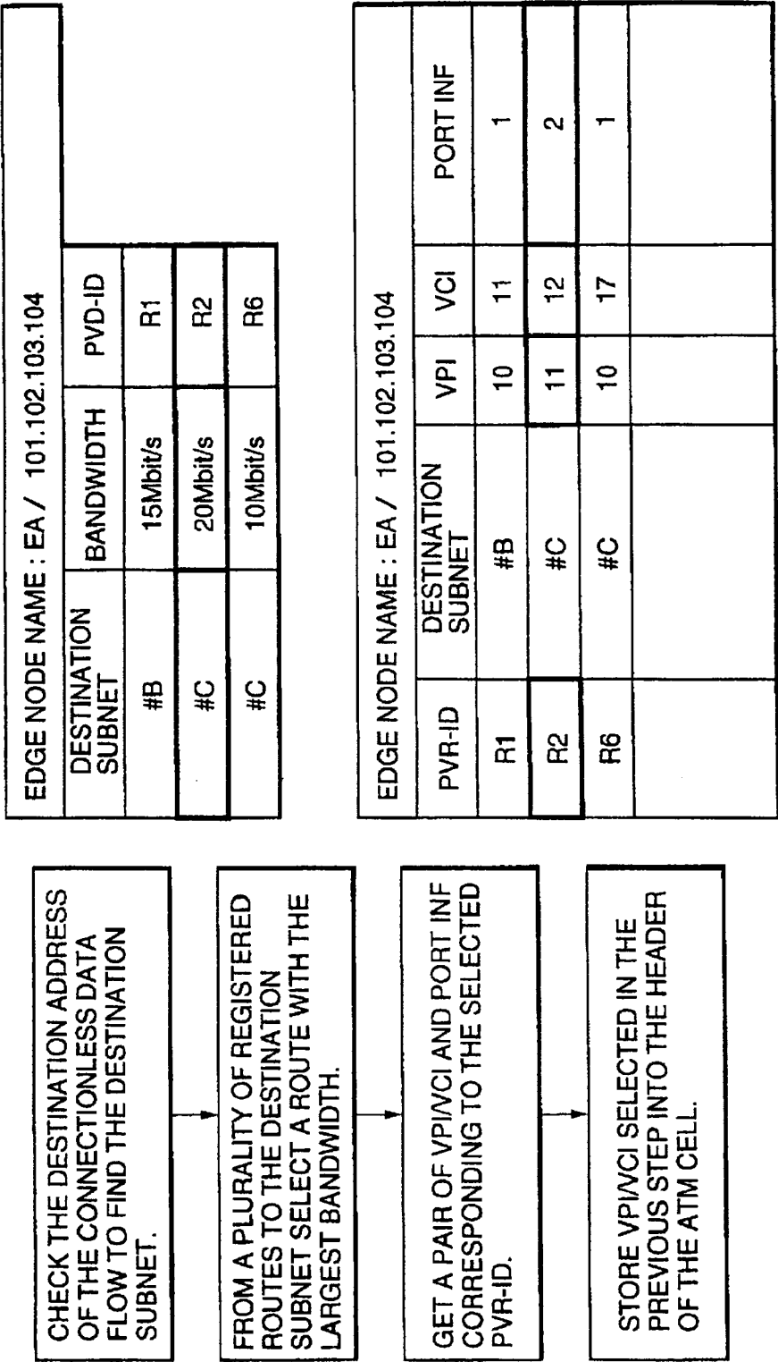
ROUTING TABLE SEARCH AND SETUP PROCEDURE USED IN EDGE NODE EA
