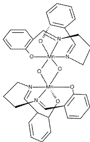
[\text{Mn}^{\text{IV}}_2(\text{salpn})(\mu\text{-O}_2)]_2
