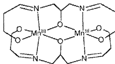
[\text{Mn}^{\text{III}}(2\text{-OHsalpn})]_2
