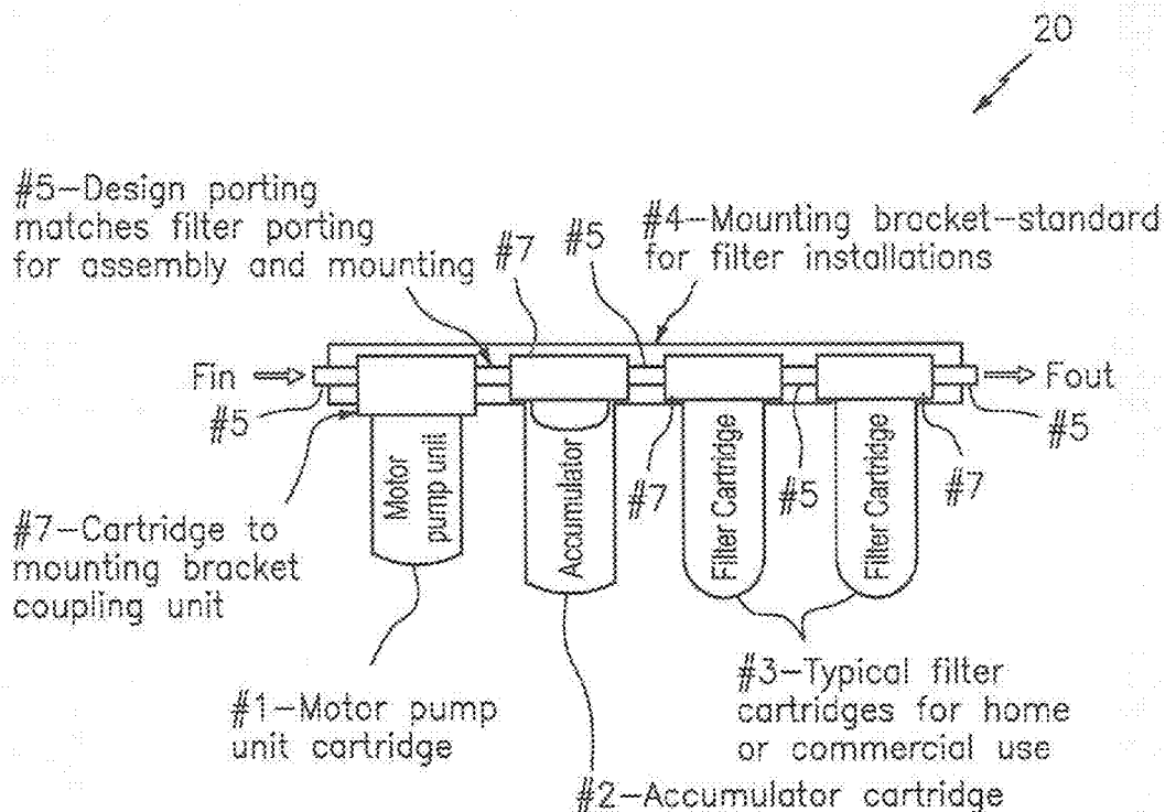
FIG. 2B: Beverage Application
