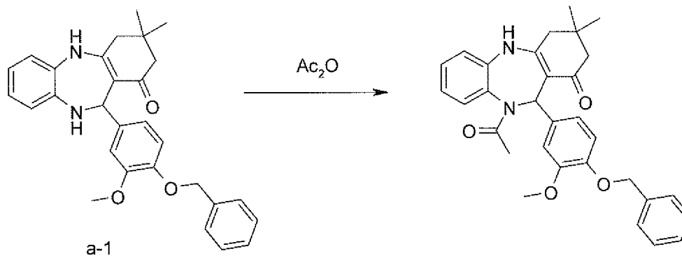
Scheme A
