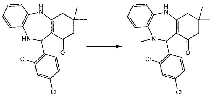
Compound 423
