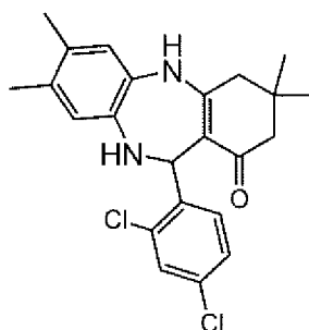
Compound 464
