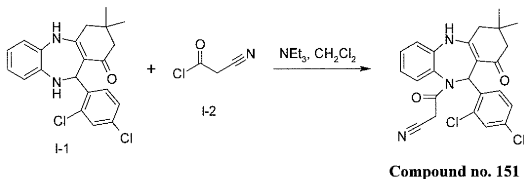
Scheme L
