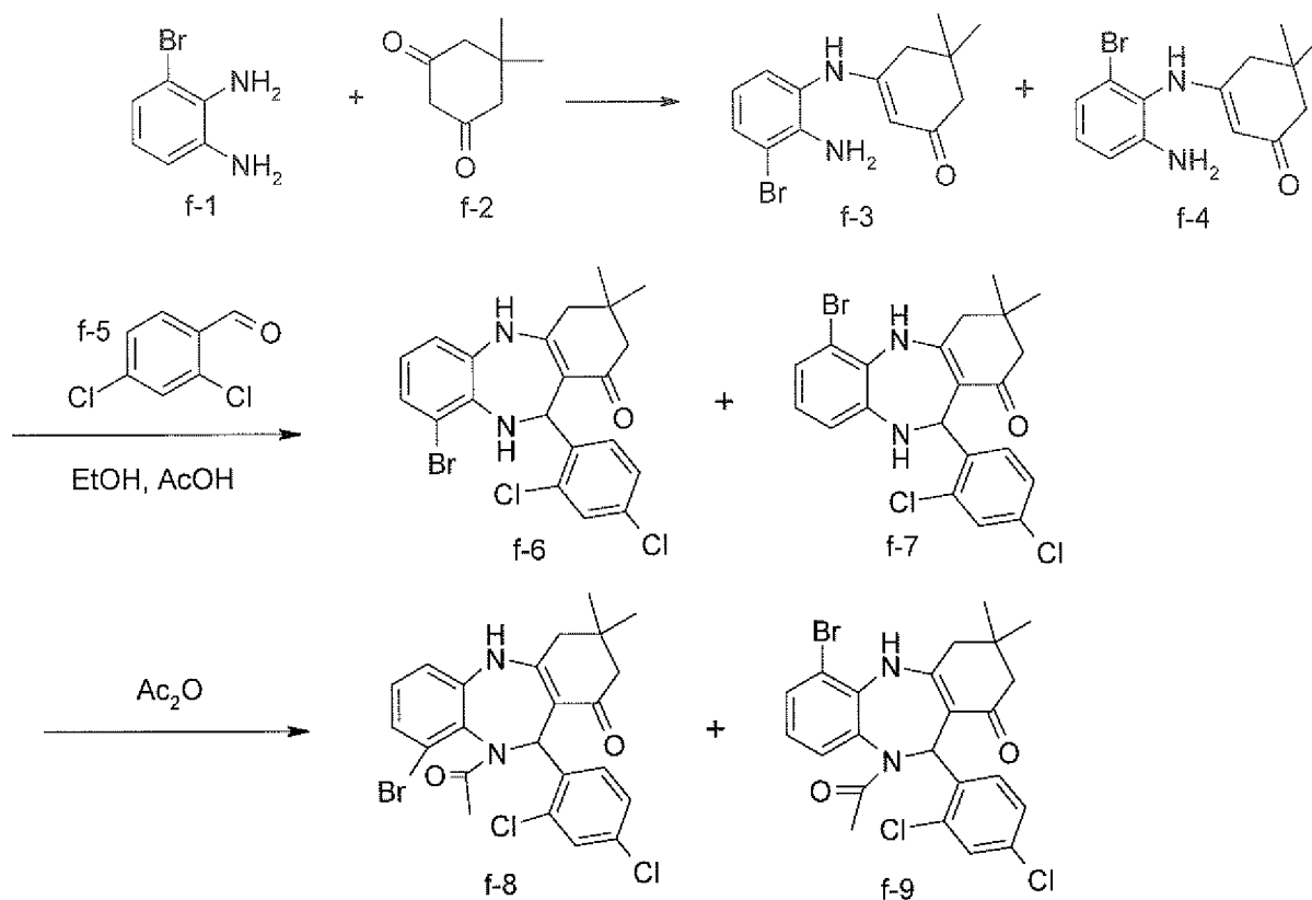
Scheme F
