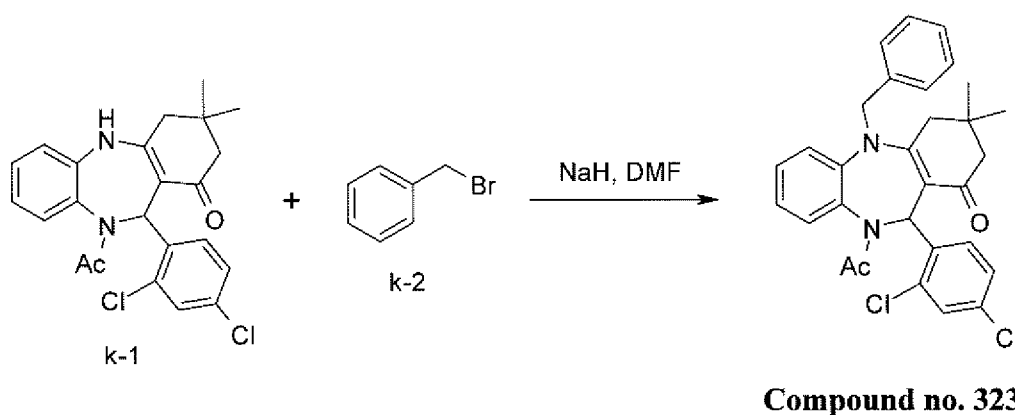
Scheme K
