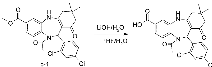
Compound no. 517
