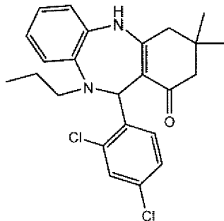
Compound 509
