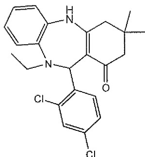
Compound 508
