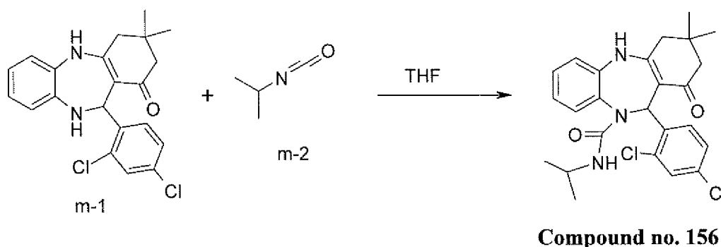
Scheme M
