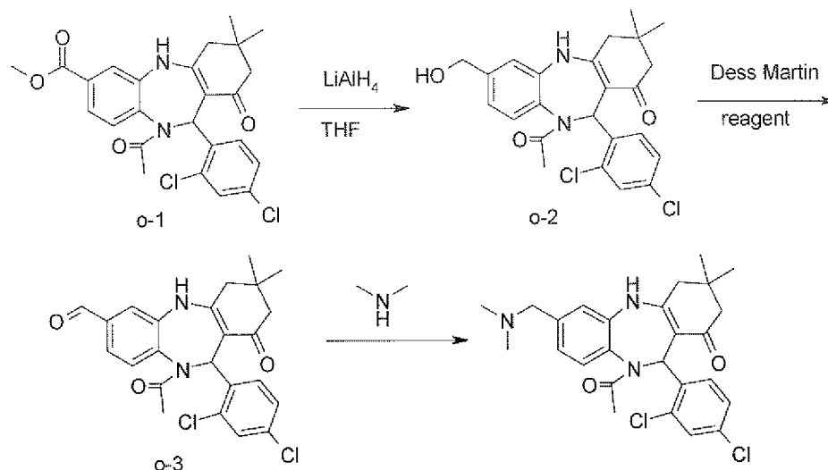
Compound no. 516
