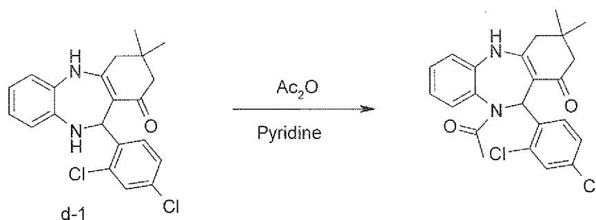
Compound no. 38
