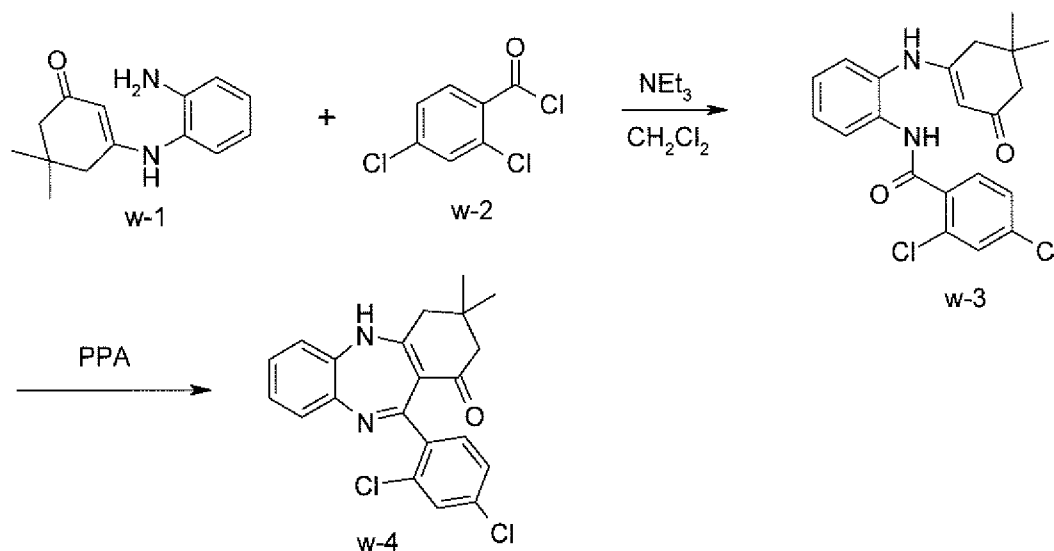
Scheme W
