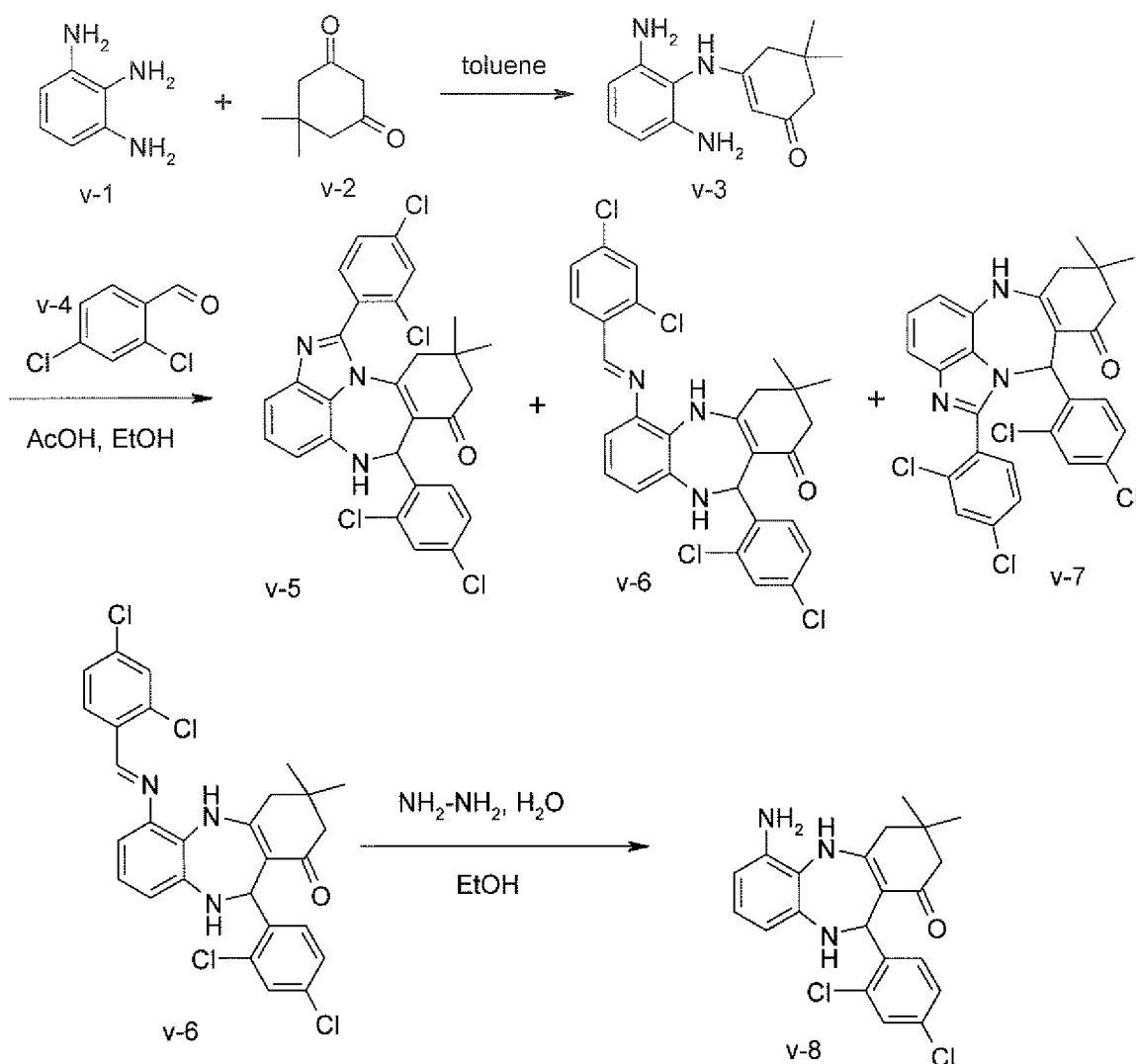
Scheme V
