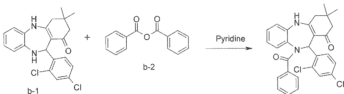
Compound no. 45
