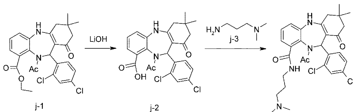
Scheme J
