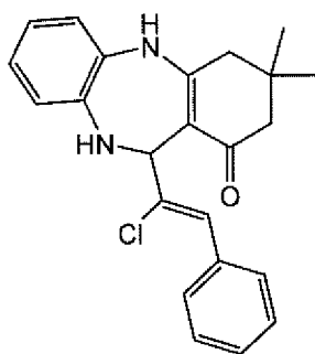
Compound 506
