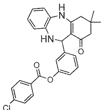
Compound 431
