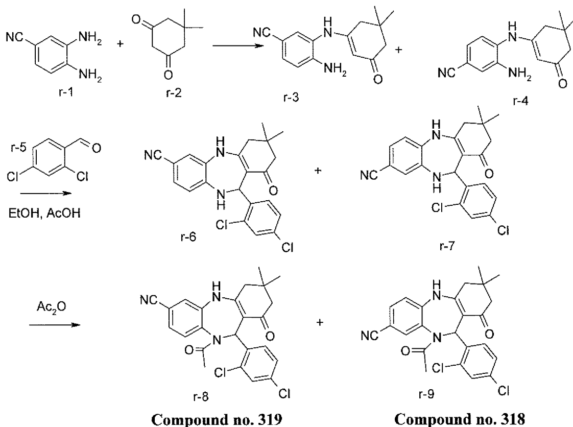
Scheme R
