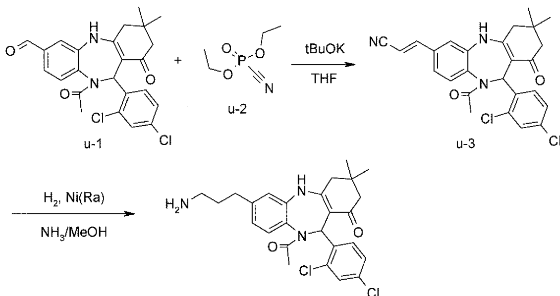
Compound no. 519
