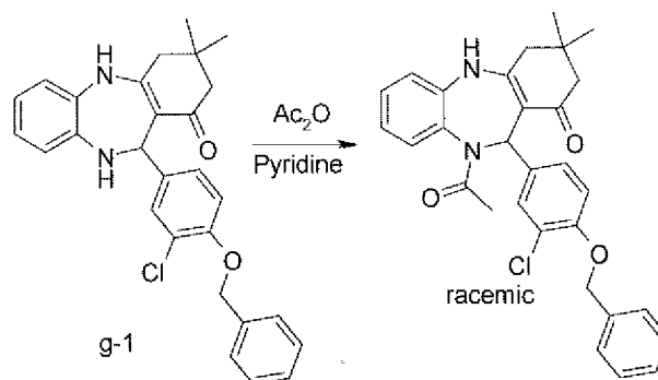
Scheme G
