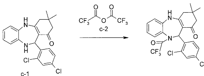
Compound no. 107
