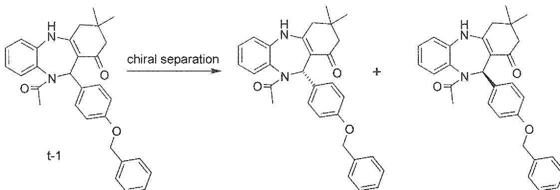
Compound no. 302
