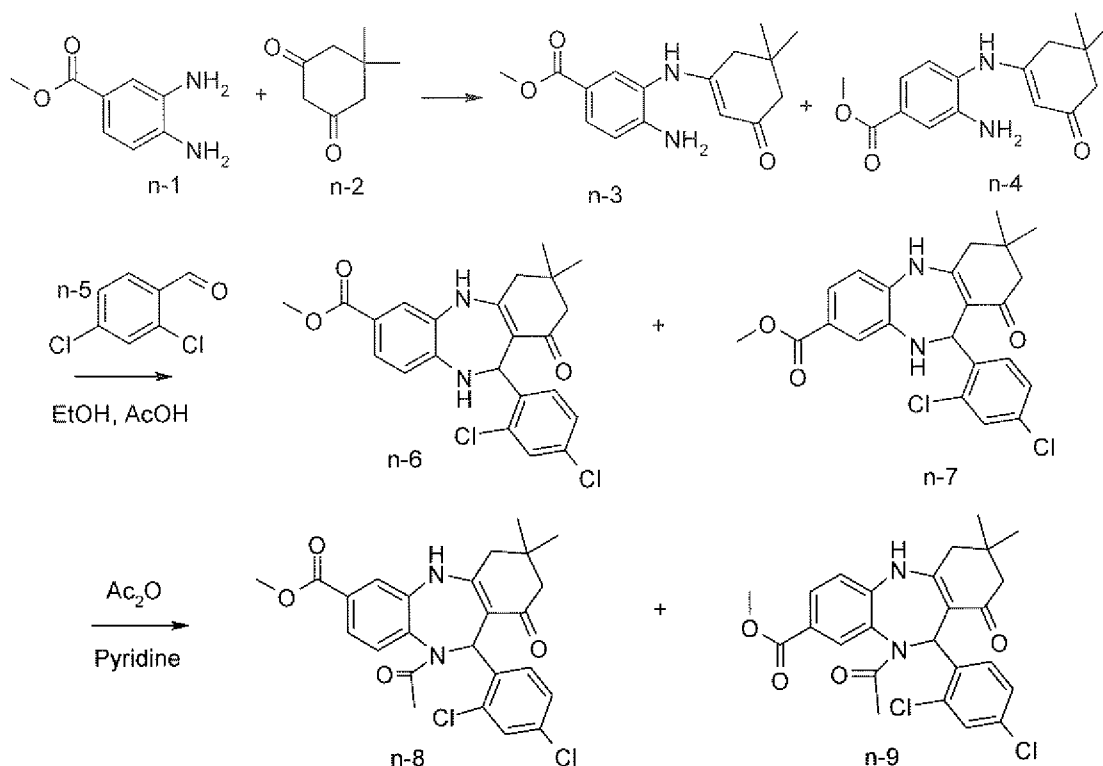
Scheme N
