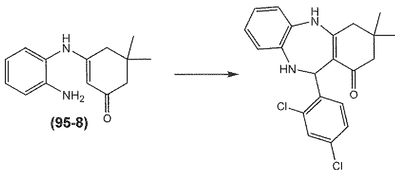
Compound 423
