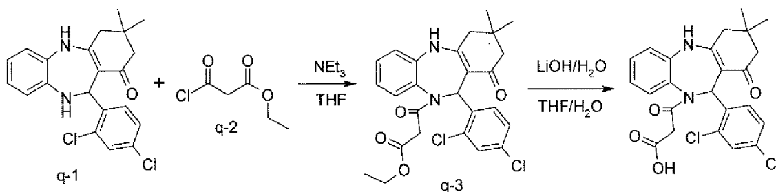
Compound no. 518
