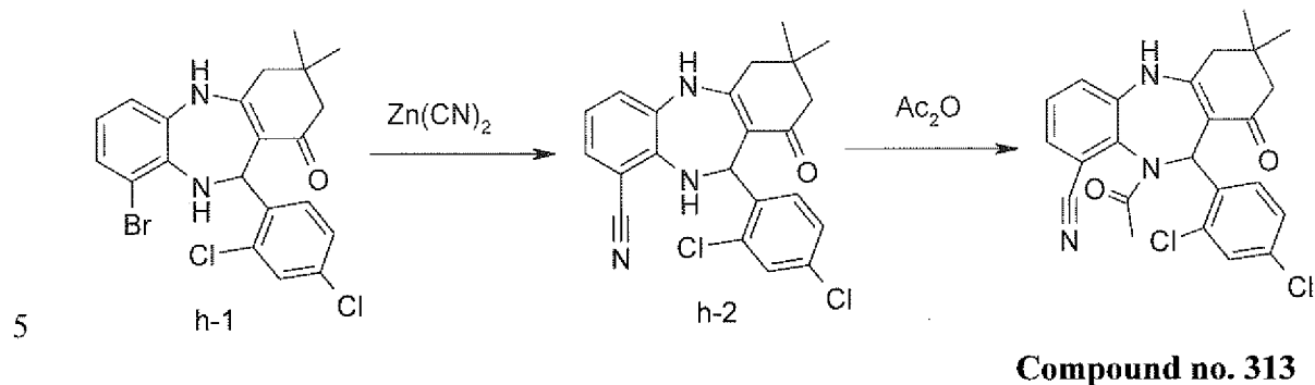
Scheme H
