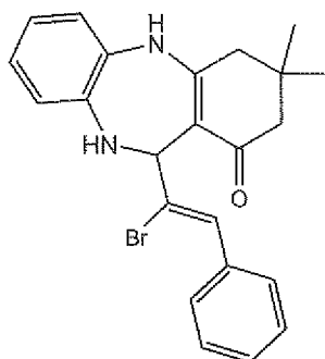
Compound 500
