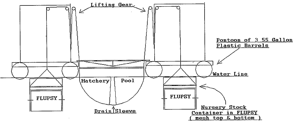
FIG. 4 - End View of 25 Spawntoon
