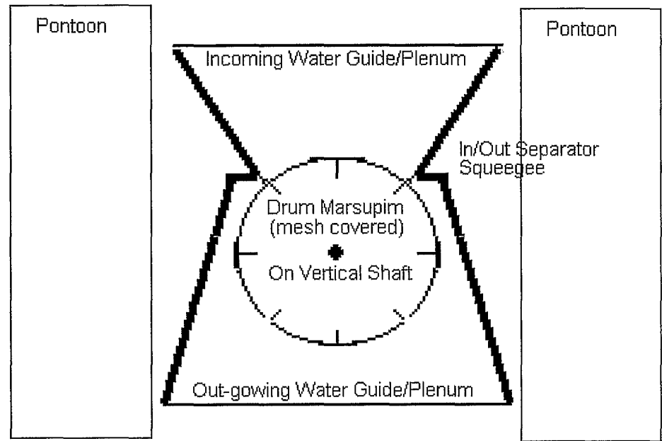
FIG. 23 – Automatic Back-Flush Marsupium (ABFM) with rotary flow control by Vertical Axis Drum TOP VIEW ( CLAIM 42 )
