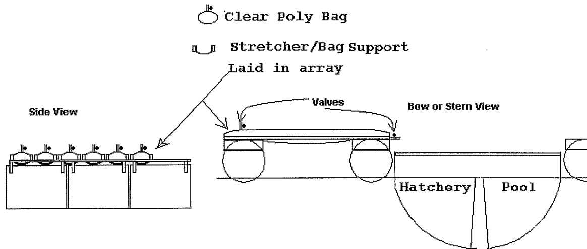
FIG. 7 – Phytoplankton Culture: Culture Bag w/fittings, Stretcher resting on two pontoons
