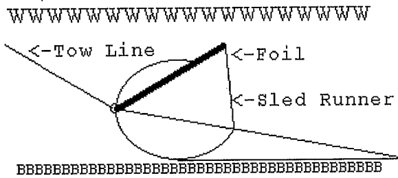
FIG. 14 – Resuspension Drag Foil of CLAIM 17
