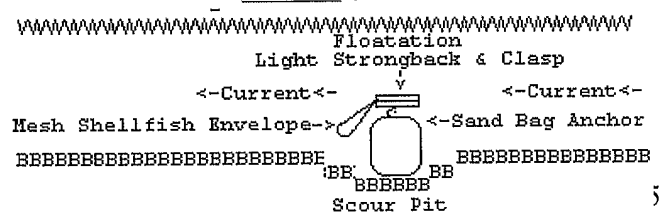
60 FIG. 17 – BUPSY of CLAIM 8 ( for low current or under possible boat traffic )
