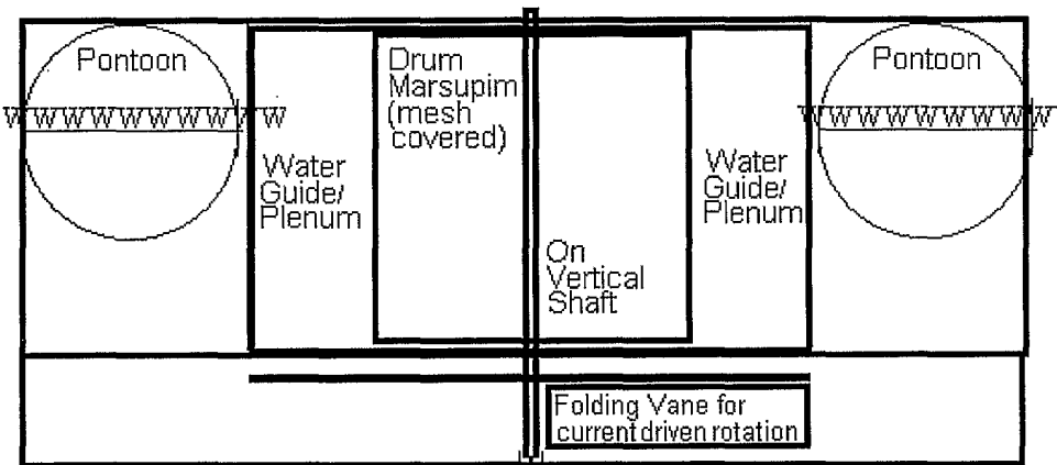
AFT VIEW
