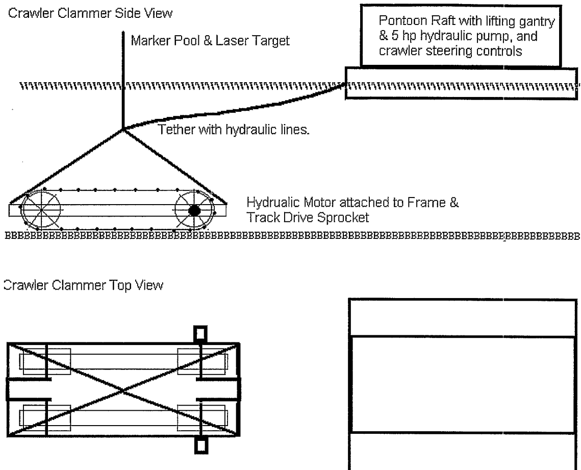
110 FIG 26 – Crawler Clammer of Claim 47
