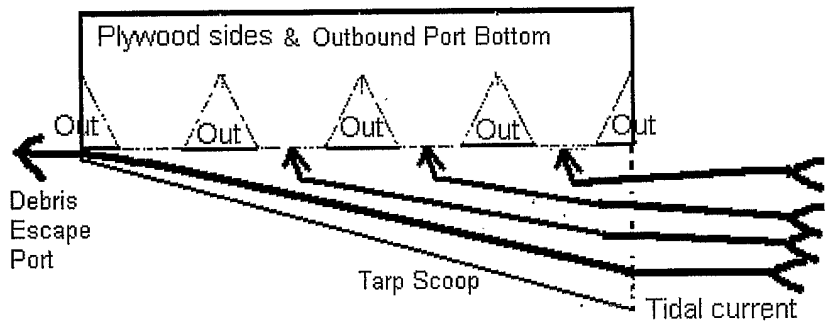
FIG. 14 – Resuspension Drag Foil of CLAIM 17
