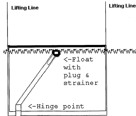
FIG. 5 – Drain Device for floating hatchery live-well
