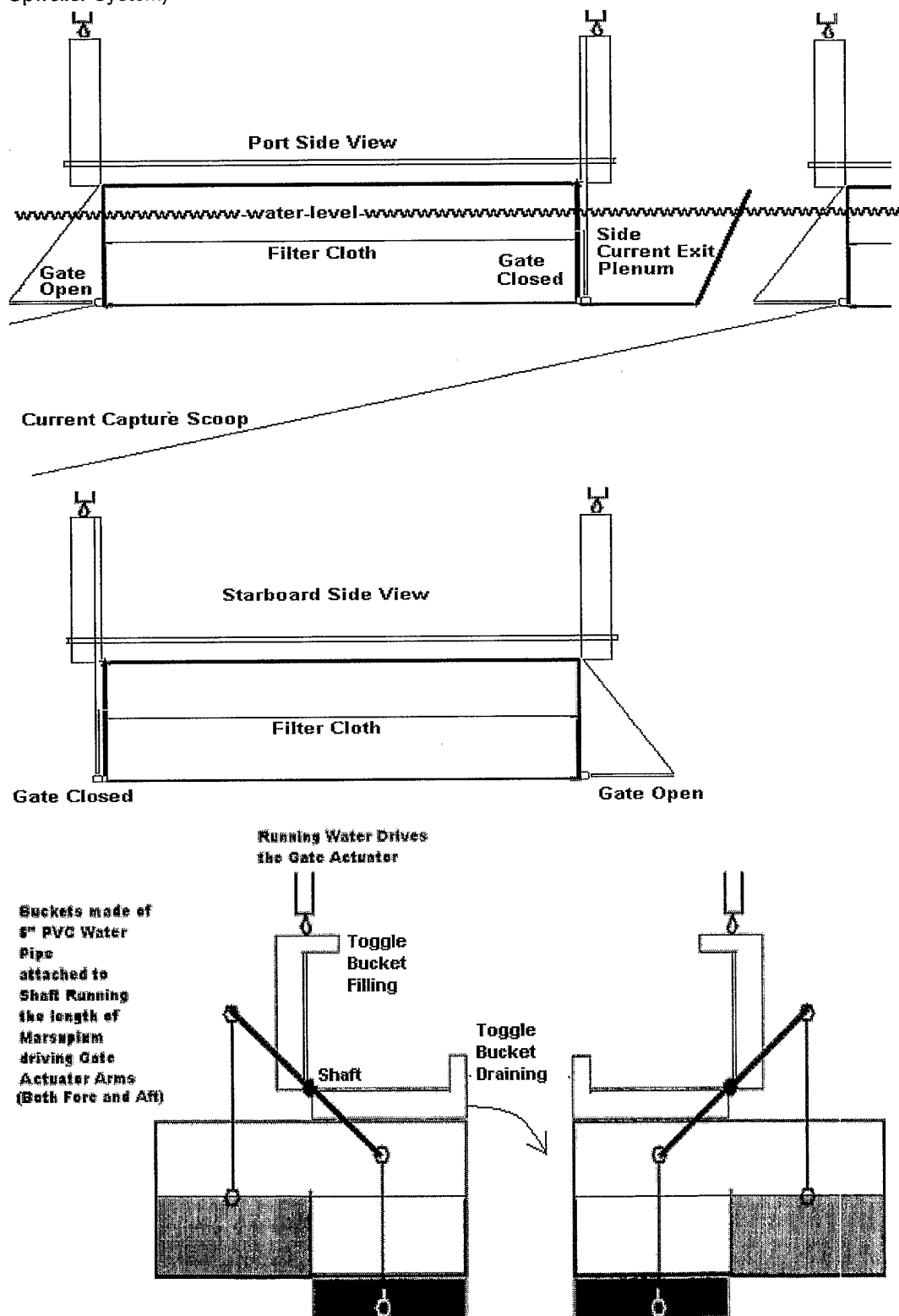
85 FIG. 21 – Series of Automated Back-flush Marsupiums (ABFM) hosted by a FLUPSY (Floating Upweller System)
