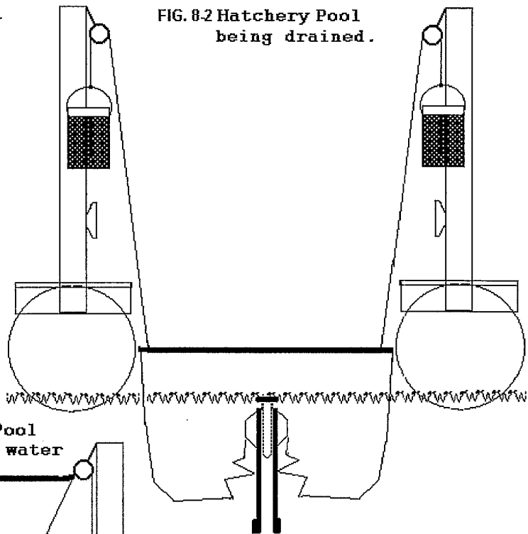
FIG. 8 Series – Hatchery Live Well Drain-Sleeve and Spawn Catcher
