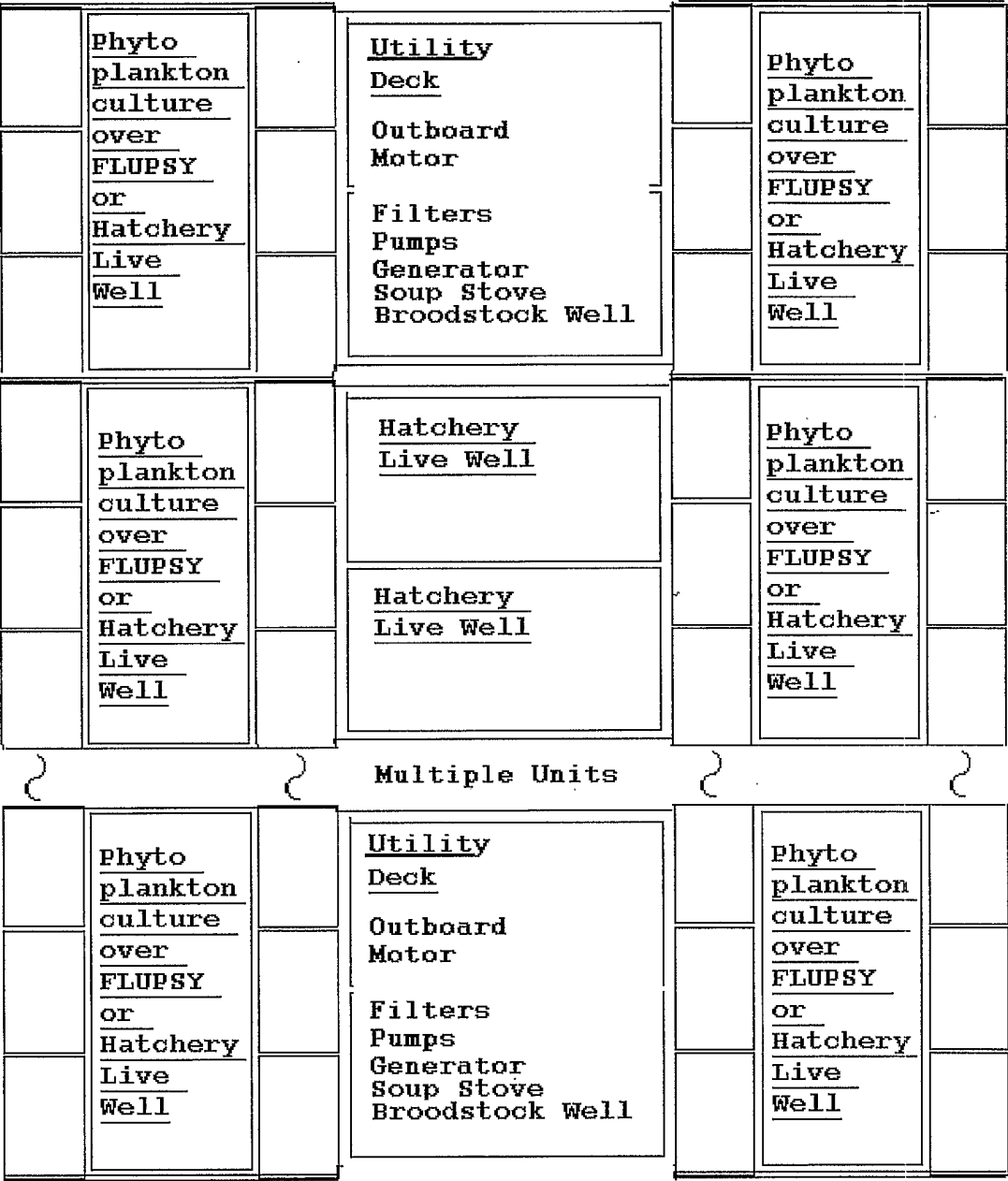
30 FIG. 6 – SpawnToon Motorboat “The Mama Cass Ostrea”
