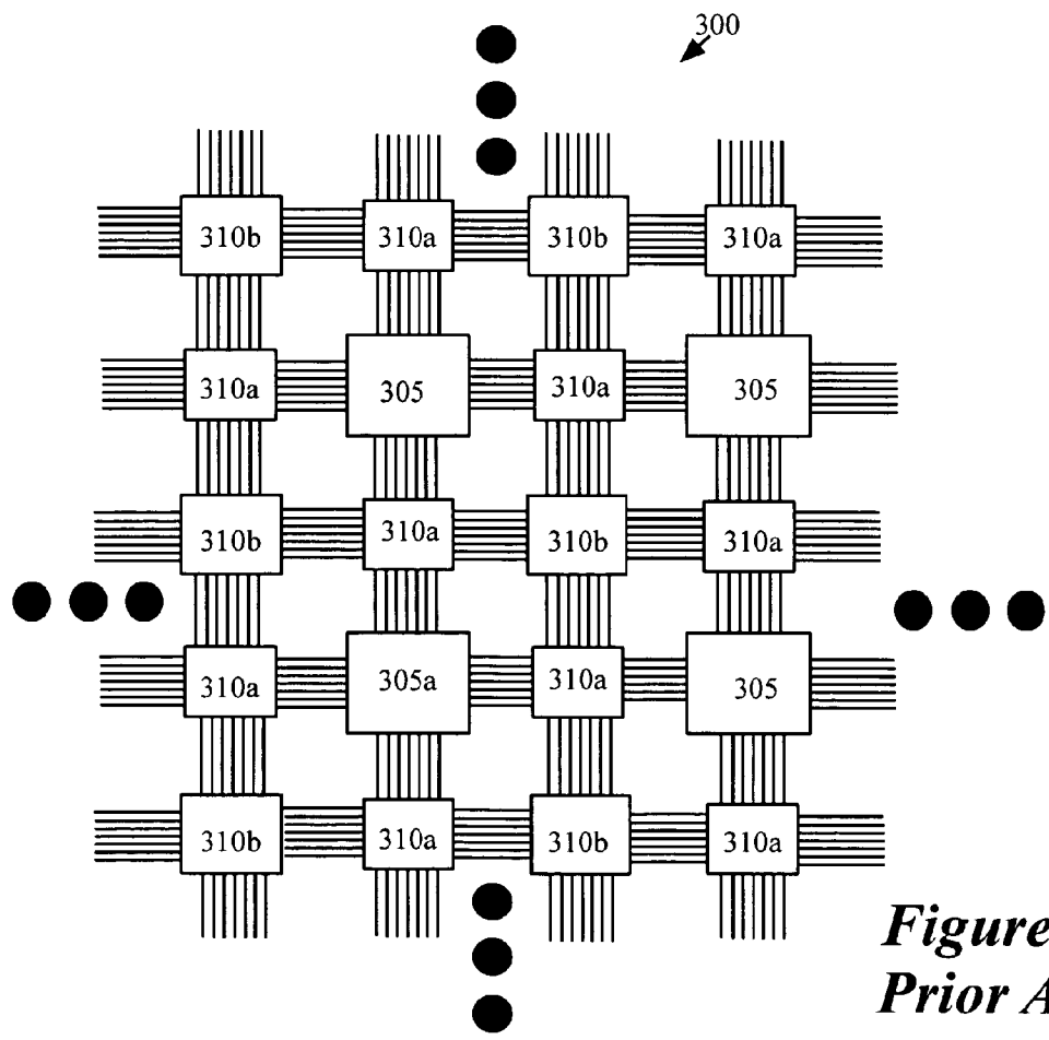
Figure 1 Prior Art
