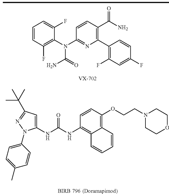
BIRB 796 (Doramapimod)
