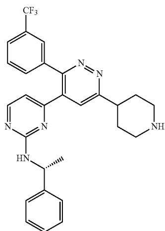
(R)-N-(1-phenylethyl)-4-(6-(piperidin-4-yl)-3-(3-(trifluoromethyl)phenyl)pyridazin-4-yl)pyrimidin-2-amine
