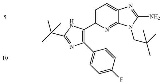
LY2228820
