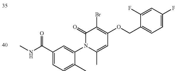
PH-797804
