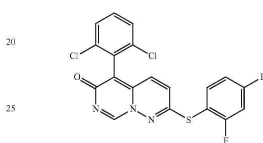
VX-745
