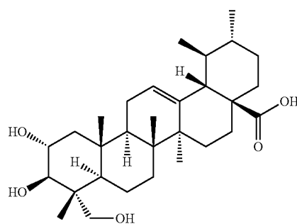
Asiatic acid
