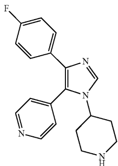
4-(4-(4-fluorophenyl)-1-(piperidin-4-yl)-1H-imidazol-5-yl)pyridine
