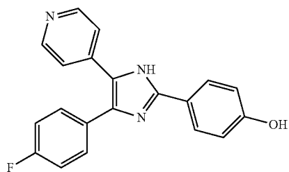
SB 202190
