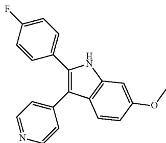
2-(4-fluorophenyl)-6-methoxy-3-(pyridin-4-yl)-1H-indole
