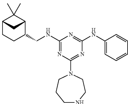
6-(1,4-diazepan-1-yl)-N²-(((1S,2R,5S)-6,6-dimethylbicyclo[3.1.1]heptan-2-yl)methyl)-N4-phenyl-1,3,5-triazine-2,4-diamine
