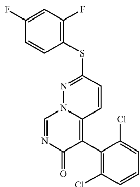
5-(2,6-dichlorophenyl)-2-(2,4-difluorophenylthio)-6H-pyrimido[1,6-b]pyridazin-6-one
