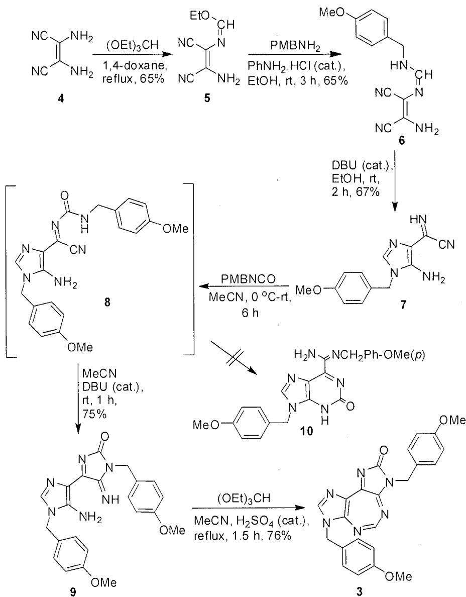
Scheme 2
