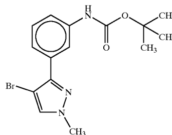
(tert-butoxy)-N-[3-(4-bromo-1-methylpyrazol-3-yl)phenyl]carboxamide
