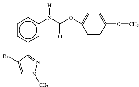
N-[3-(4-bromo-1-methylpyrazol-3-yl)phenyl][4-methoxyphenoxy]carboxamide
