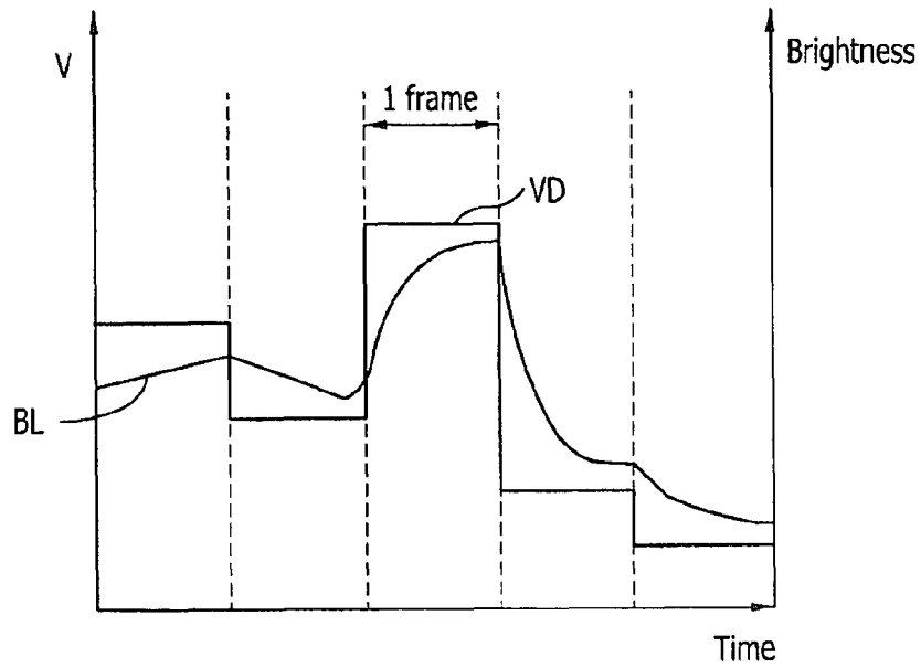
FIG. 2 Related Art
