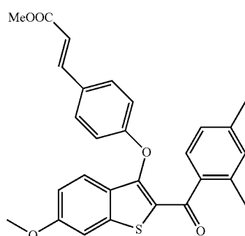
Methyl (E)-3-4-((2-(2,4-dimethylbenzoyl)-6-methoxybenzo[b]thiophen-3-yl)oxy)phenyl)acrylate
