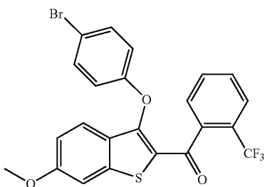
(3-(4-bromophenoxy)-6-methoxybenzo[b]thiophen-2-yl)(2-(trifluoromethyl)phenyl)methanone
