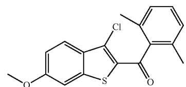
(3-Chloro-6-methoxybenzo[b]thiophen-2-yl)(2,6-dimethylphenyl)methanone
