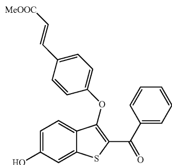
Methyl (E)-3-((2-benzoyl-6-hydroxybenzo[b]thiophen-3-yl)oxy)phenyl)acrylate
