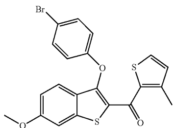
(3-(4-bromophenoxy)-6-methoxybenzo[b]thiophen-2-yl)(3-methylthiophen-2-yl)methanone
