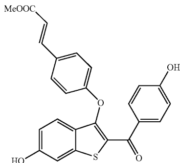
Methyl (E)-3-(4-((6-hydroxy-2-(4-hydroxybenzoyl)benzo[b]thiophen-3-yl)oxy)phenyl)acrylate
