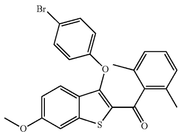
(3-(4-bromophenoxy)-6-methoxybenzo[b]thiophen-2-yl)(2,6-dimethylphenyl)methanone
