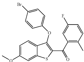
(3-(4-bromophenoxy)-6-methoxybenzo[b]thiophen-2-yl)(5-fluoro-2-methylphenyl)methanone
