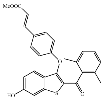
Methyl (E)-3-(4-((2-(2,6-dimethylbenzoyl)-6-hydroxybenzo[b]thiophen-3-yl)oxy)phenyl)acrylate
