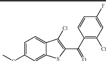
(2-Chloro-4-fluorophenyl)(3-chloro-6-methoxybenzo[b]thiophen-2-yl)methanone
