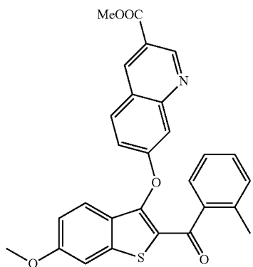
Methyl 7-((6-methoxy-2-(2-methylbenzoyl)benzo[b]thiophen-3-yl)oxy)quinoline-3-carboxylate
