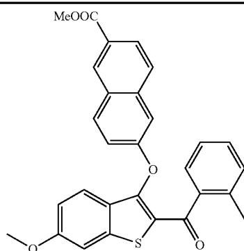
Methyl 6-((6-methoxy-2-((2-methylbenzoyl)benzo[b]thiophen-3-yl)oxy)-2-naphthoate
