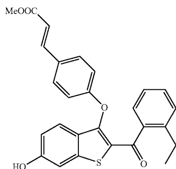
Methyl (E)-3-((2-(2-ethylbenzoyl)-6-hydroxybenzo[b]thiophen-3-yl)oxy)phenyl)acrylate
