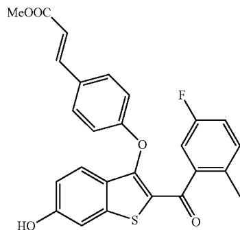
Methyl (E)-3-((2-(5-fluoro-2-methylbenzoyl)-6-hydroxybenzo[b]thiophen-3-yl)oxy)phenyl)acrylate
