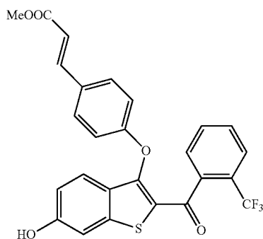
Methyl (E)-3-(4-((6-hydroxy-2-(2-(trifluoromethyl)benzoyl)benzo[b]thiophen-3-yl)oxy)phenyl)acrylate
