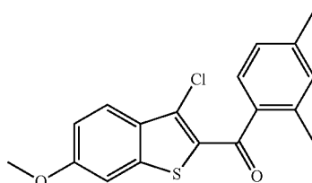
(3-chloro-6-methoxybenzo[b]thiophen-2-yl)(2,4-dimethylphenyl)methanone
