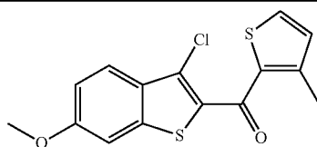
(3-chloro-6-methoxybenzo[b]thiophen-2-yl)(3-methylthiophen-2-yl)methanone
