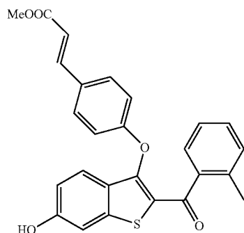
Methyl (E)-3-((6-hydroxy-2-(2-methylbenzoyl)benzo[b]thiophen-3-yl)oxy)phenyl)acrylate
