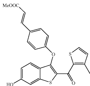
Methyl (E)-3-(4-((6-hydroxy-2-(3-methylthiophene-2-carbonyl)benzo[b]thiophen-3-yl)oxy)phenyl)acrylate
