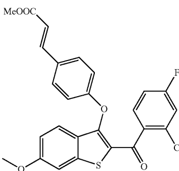
Methyl (E)-3-4-((2-(2-chloro-4-fluorobenzoyl)-6-methoxybenzo[b]thiophen-3-yl)oxy)phenyl)acrylate
