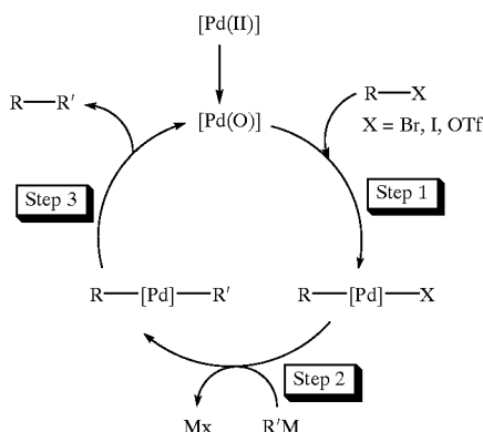
Scheme 2. Catalytic cycle for the cross-coupling organo-halides or -triflates with organometallics.
