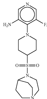
4-(4-(1,4-diazabicyclo[3.2.2]nonan-4-ylsulfonyl)piperidin-1-yl)-5-fluoropyridin-3-amine:
