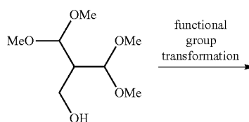
Scheme 3—Preparation of butanenitrile intermediates
