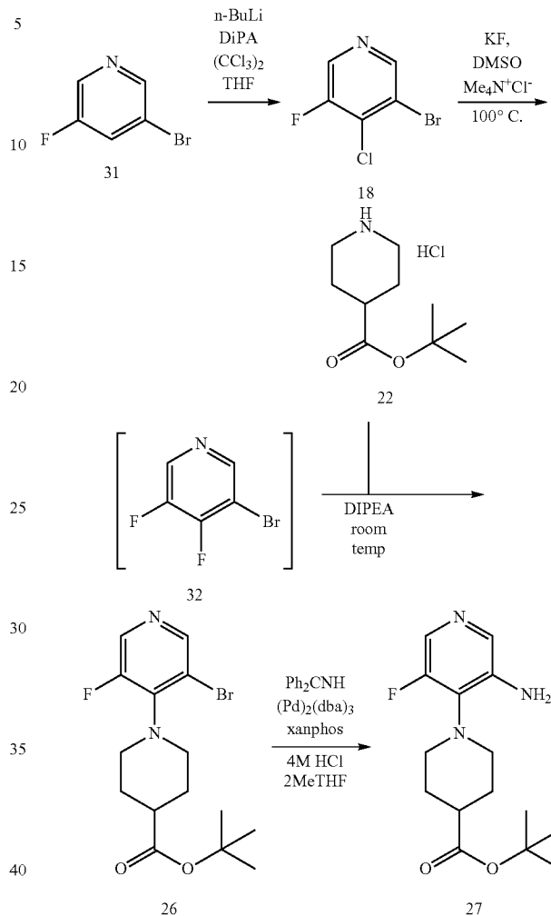
Scheme 7b: Alternative synthesis of tert-butyl 1-(3-amino-5-fluoro-4-pyridyl)piperidine-4-carboxylate
