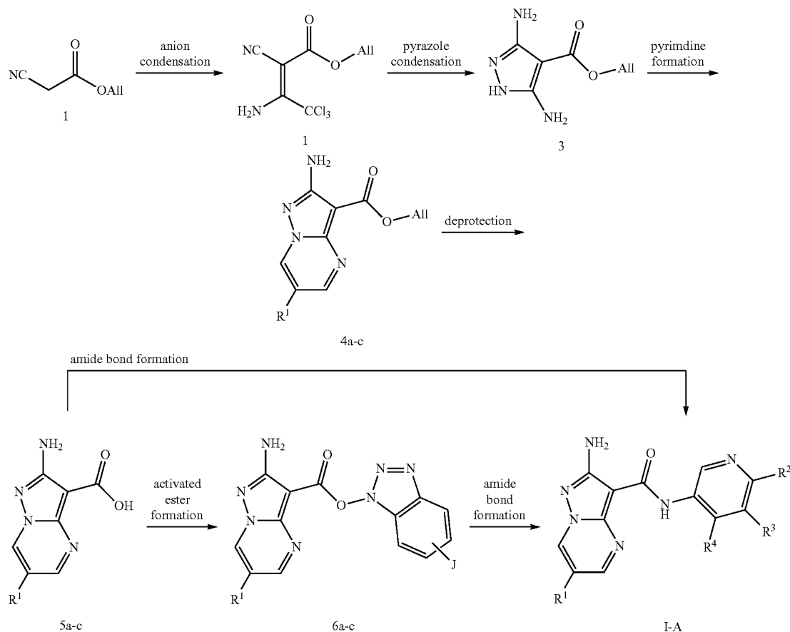
Scheme 1: General approach for the preparation of compounds I-A
