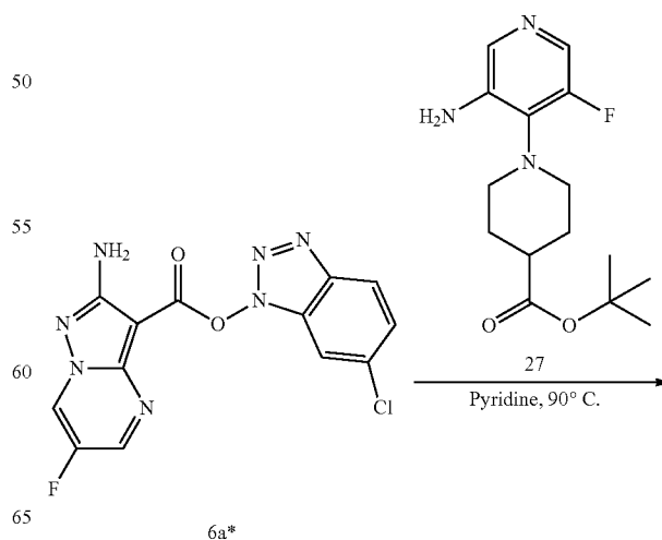
Scheme 2c: Alternative approach to prepare compound I-G-32
