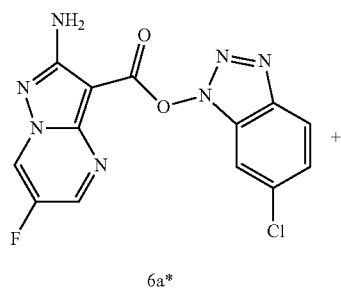
Scheme 2b: Preparation of compound I-G-32
