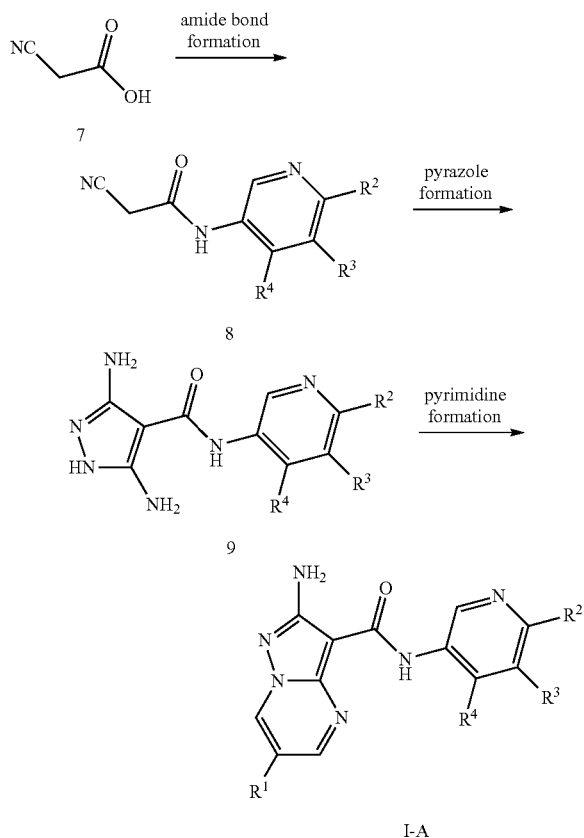
Scheme 2: Alternative approach for the preparation of compounds I-A
