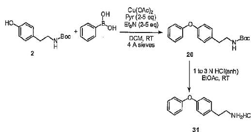
Scheme 4: Synthesis of Phenyl Derivative
