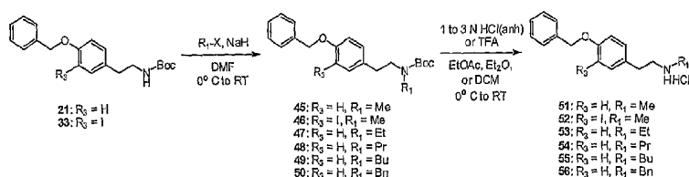
Scheme 6: Synthesis of N-Alkylated Derivatives
