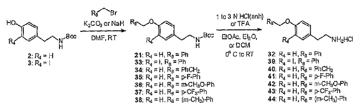
Scheme 5: Synthesis of O-Alkylated Tyramine Derivatives
