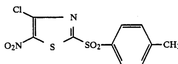
(Compound No. 66)
