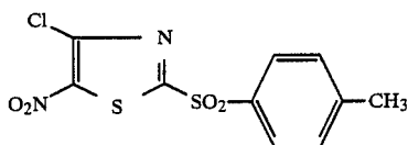
(Compound No. 66)
