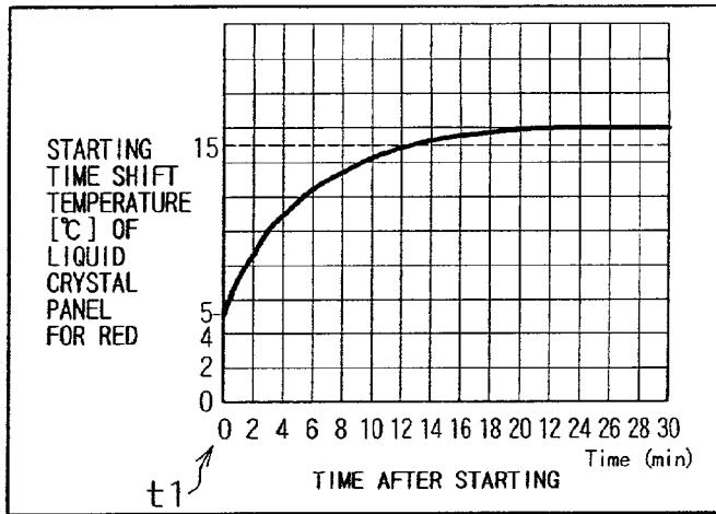
DATA OF STARTING TIME SHIFT TEMPERATURE (TS) (FOR RED)
